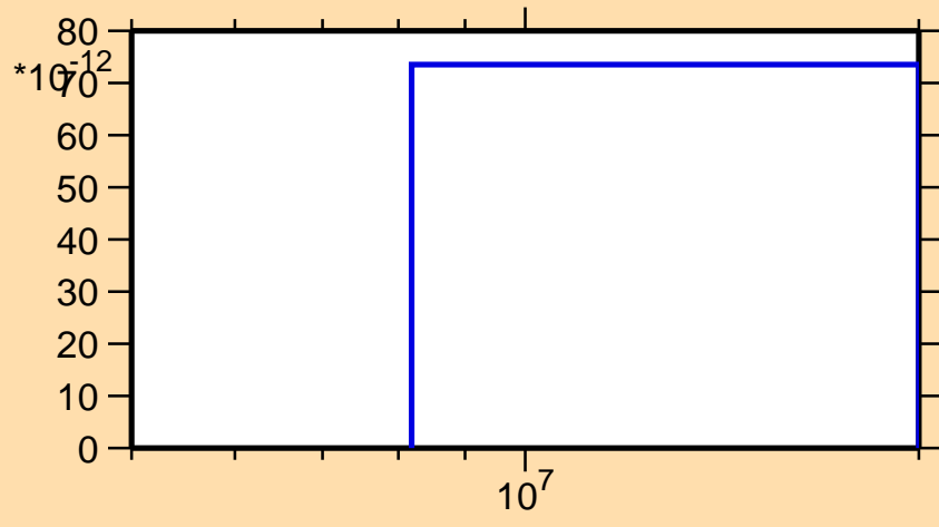
\sigma vs. E for ^{208}\text{Bi}(n,p\alpha)
