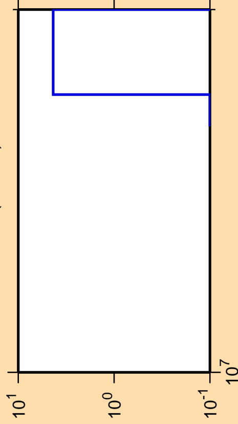
\Delta\sigma/\sigma vs. E for ^{209}\text{Bi}(n,3n\alpha)
