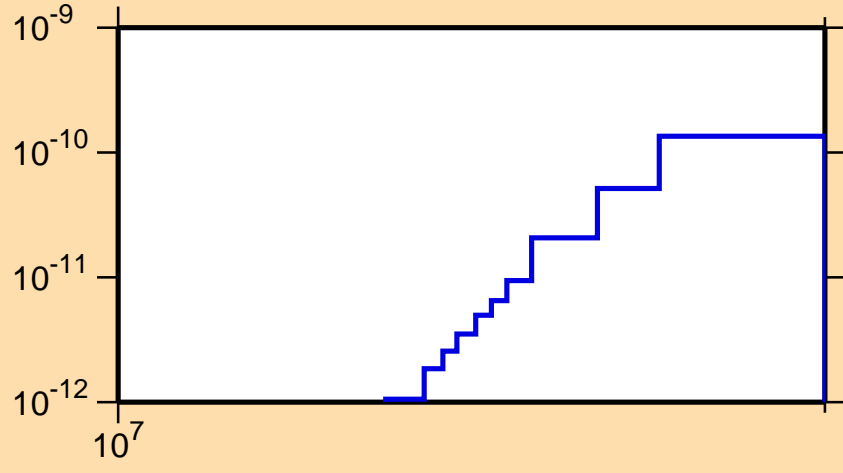
\sigma vs. E for ^{209}\text{Bi}(n,p\alpha)
