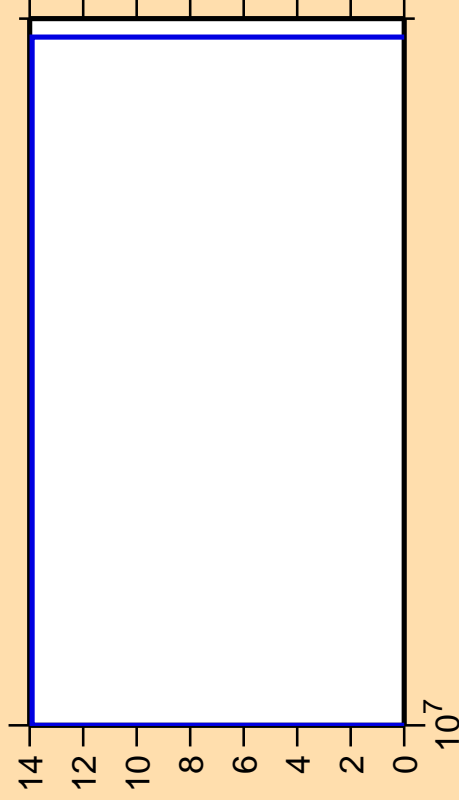
\Delta\sigma/\sigma vs. E for ^{209}\text{Bi}(n,3n)
