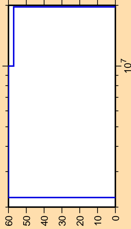
\Delta\sigma/\sigma vs. E for ^{209}\text{Bi}(n,n\alpha)
