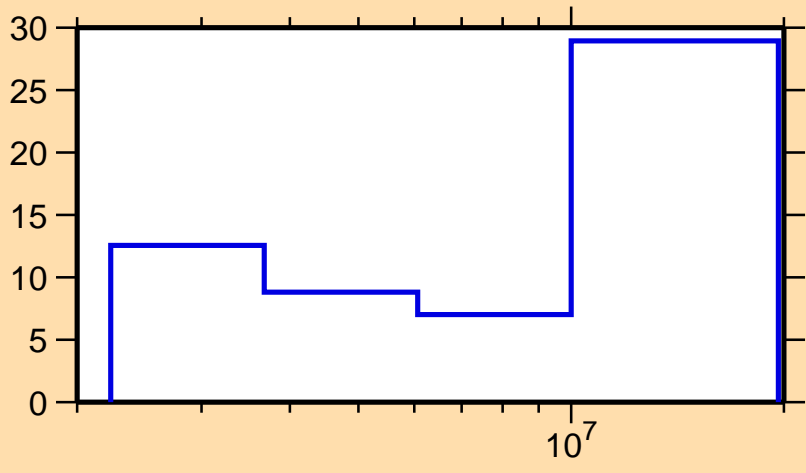
\Delta\sigma/\sigma vs. E for ^{209}\text{Bi}(n,n\text{cont.})
