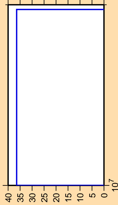
\Delta\sigma/\sigma vs. E for ^{209}\text{Bi}(n,p\alpha)
