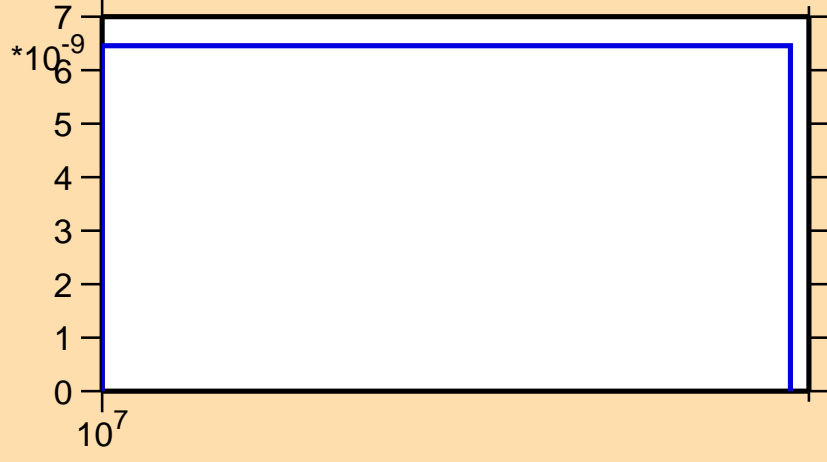
\sigma vs. E for ^{209}\text{Bi}(n,nt)
