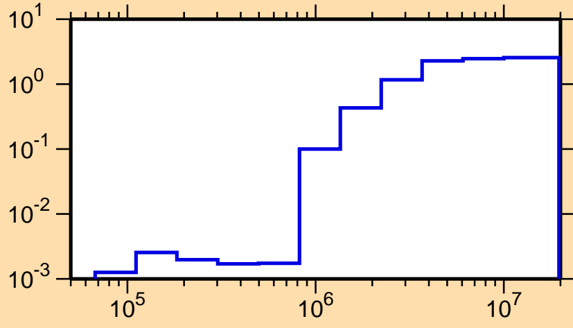
\sigma vs. E for ^{209}\text{Bi}(n,\text{nonel.})
