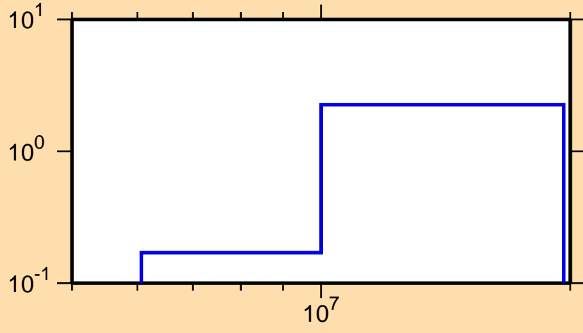
\sigma vs. E for ^{209}\text{Bi}(n,2n)
