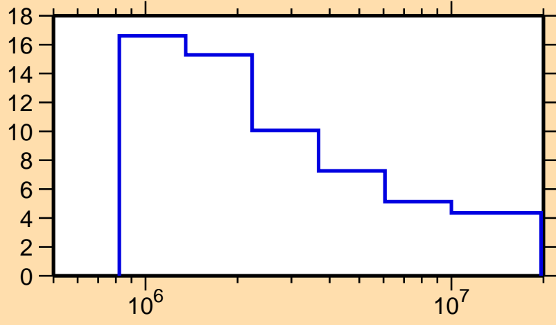
\Delta\sigma/\sigma vs. E for ^{209}\text{Bi}(n,\text{nonel.})
