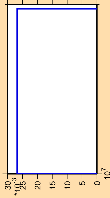
\Delta\sigma/\sigma vs. E for ^{209}\text{Bi}(n,3n\alpha)
