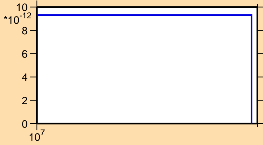
\sigma vs. E for ^{209}\text{Bi}(n,p\alpha)
