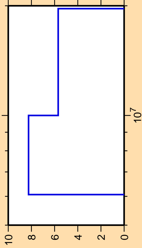
\Delta\sigma/\sigma vs. E for ^{209}\text{Bi}(n,2n)
