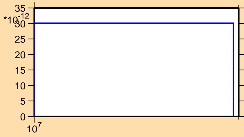
\sigma vs. E for ^{209}\text{Bi}(n,\text{He}3)
