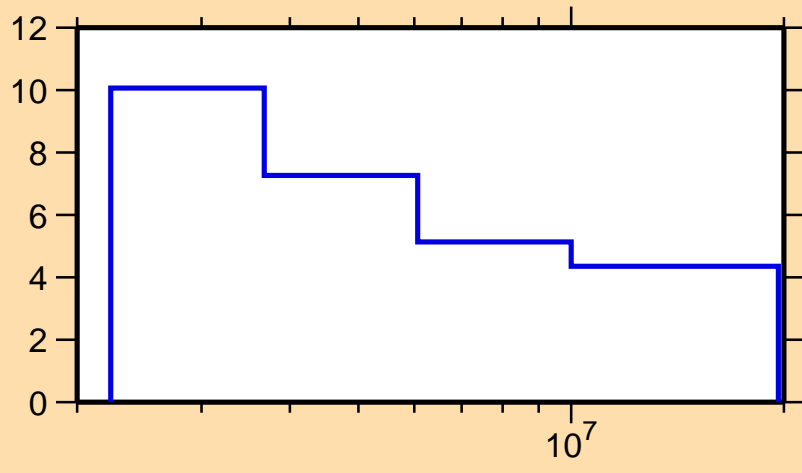
\Delta\sigma/\sigma vs. E for ^{209}\text{Bi}(n,n\text{nonel.})
