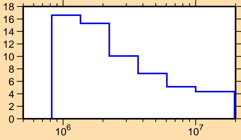
\Delta\sigma/\sigma vs. E for ^{209}\text{Bi}(n,\text{nonel.})
