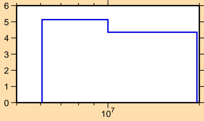
\Delta\sigma/\sigma vs. E for ^{209}\text{Bi}(n,\text{nonel.})
