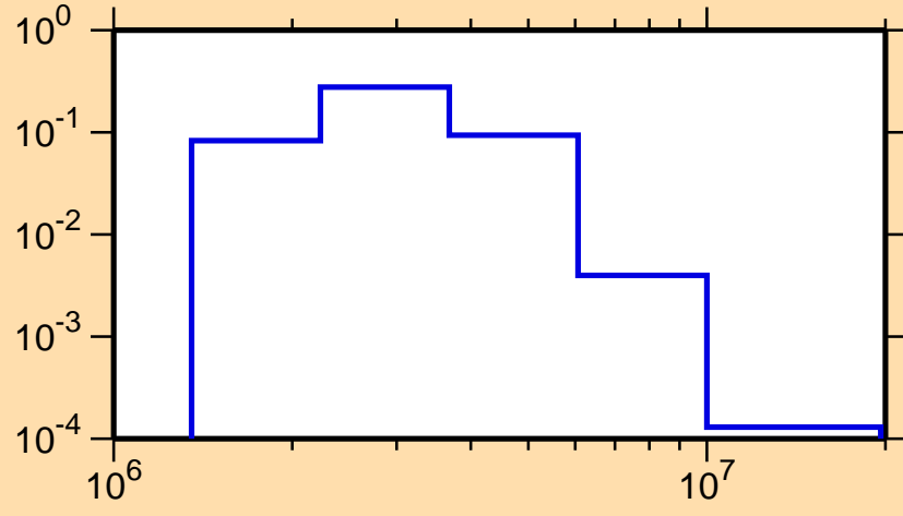
\sigma vs. E for ^{209}\text{Bi}(n,n_2)
