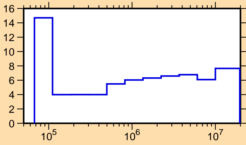
\Delta\sigma/\sigma vs. E for ^{209}\text{Bi}(n,\text{el.})
