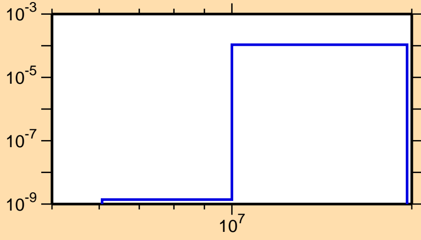
\sigma vs. E for ^{209}\text{Bi}(n,t)
