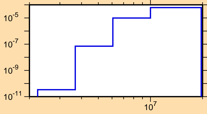
\sigma vs. E for ^{209}\text{Bi}(n,n\alpha)
