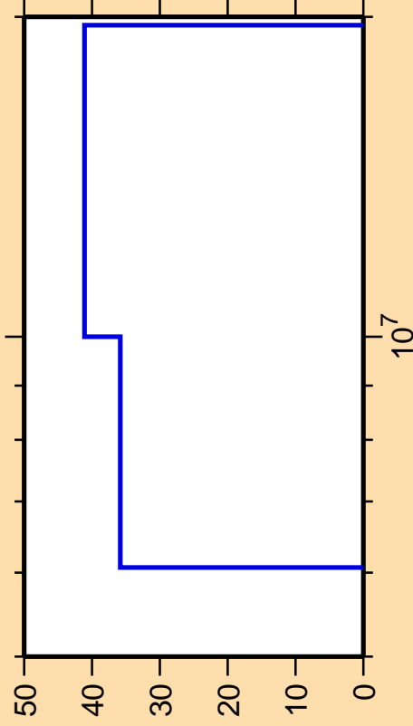
\Delta\sigma/\sigma vs. E for ^{209}\text{Bi}(n,p)
