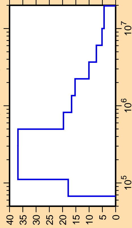
\Delta\sigma/\sigma vs. E for ^{209}\text{Bi}(n,\text{nonel.})
