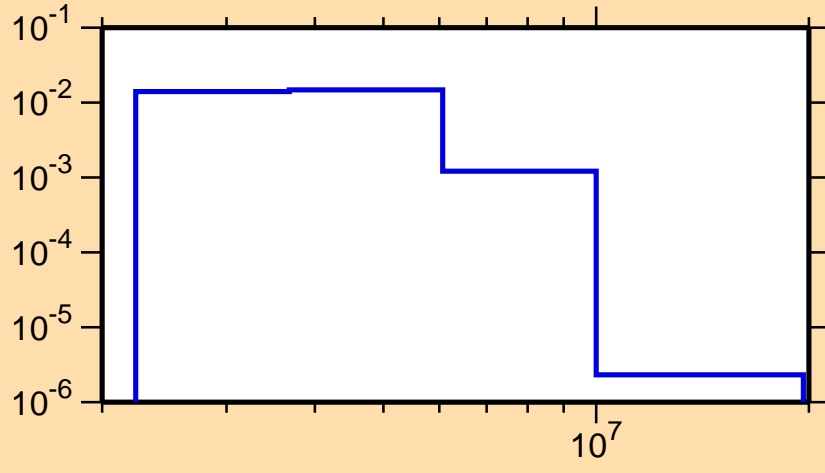
\sigma vs. E for ^{209}\text{Bi}(n,n_4)
