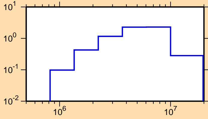
\sigma vs. E for ^{209}\text{Bi}(n,\text{inel.})
