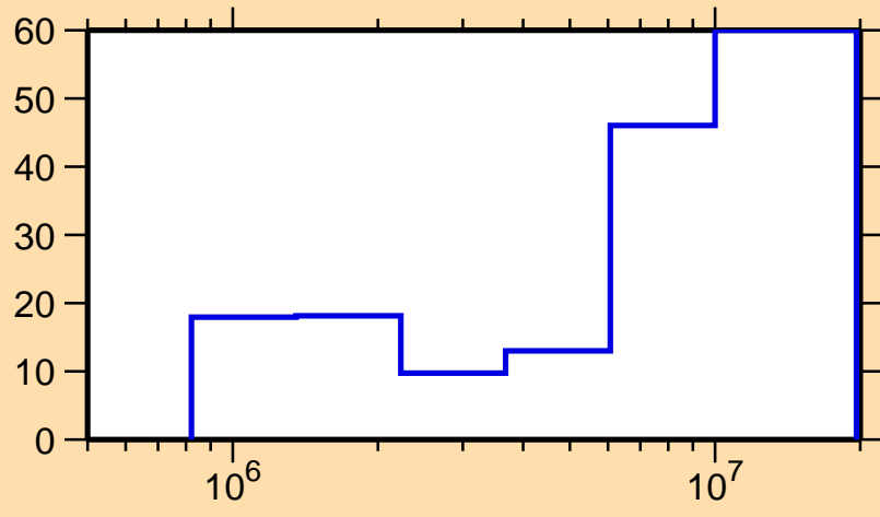
\Delta\sigma/\sigma vs. E for ^{209}\text{Bi}(n,n_1)
