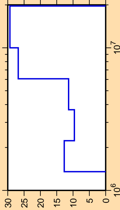
\Delta\sigma/\sigma vs. E for ^{209}\text{Bi}(n,n_2)
