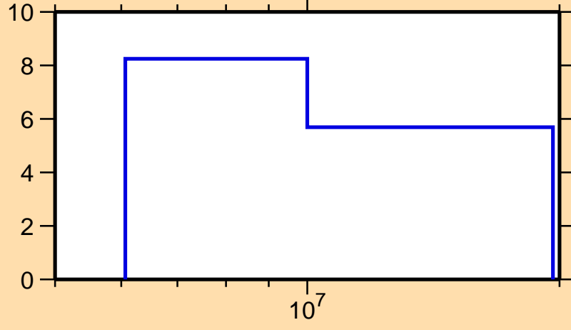
\Delta\sigma/\sigma vs. E for ^{209}\text{Bi}(n,2n)
