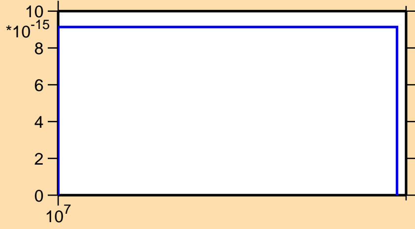
\sigma vs. E for ^{209}\text{Bi}(n,3n\alpha)
