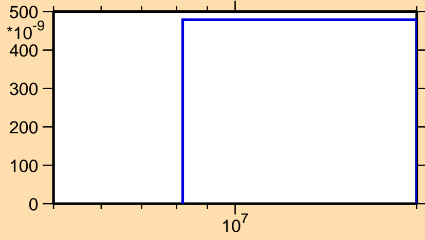
\sigma vs. E for ^{209}\text{Bi}(n,2n\alpha)
