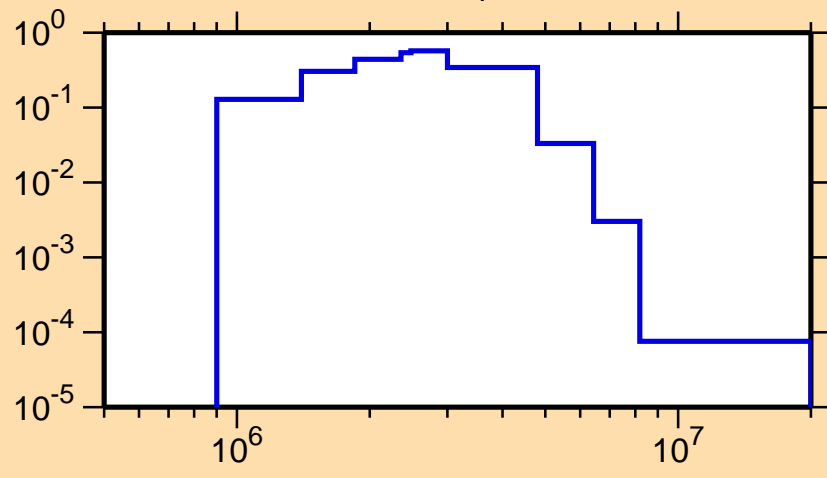
\sigma vs. E for ^{209}\text{Bi}(n,n_1)
