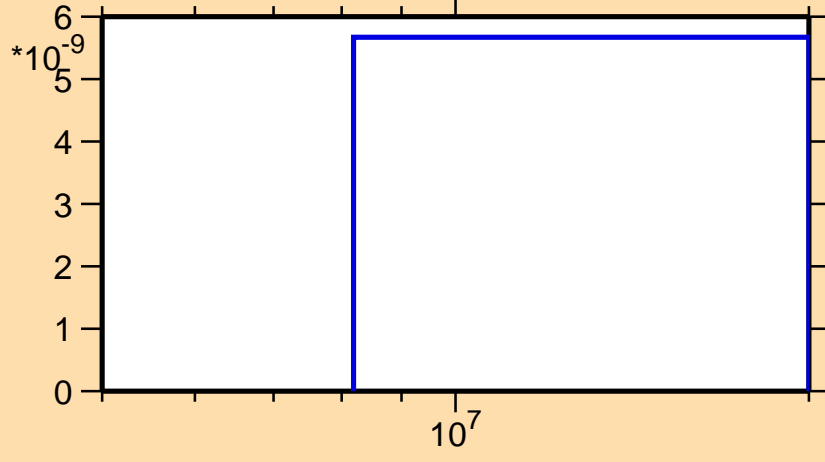
\sigma vs. E for ^{209}\text{Bi}(n,nt)
