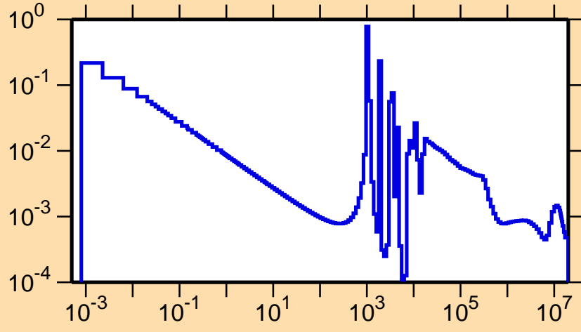
\sigma vs. E for ^{210}\text{Bi}(n,\gamma)
