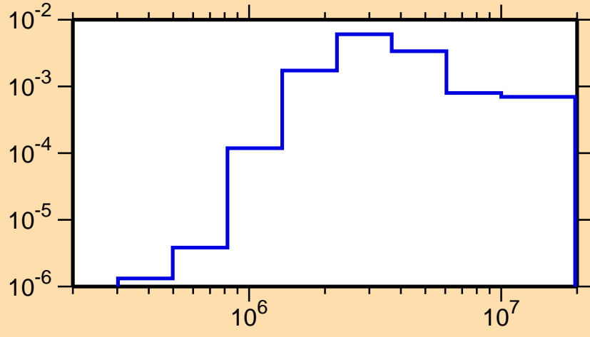
\sigma vs. E for ^{210}\text{Bi}(n,n_2)
