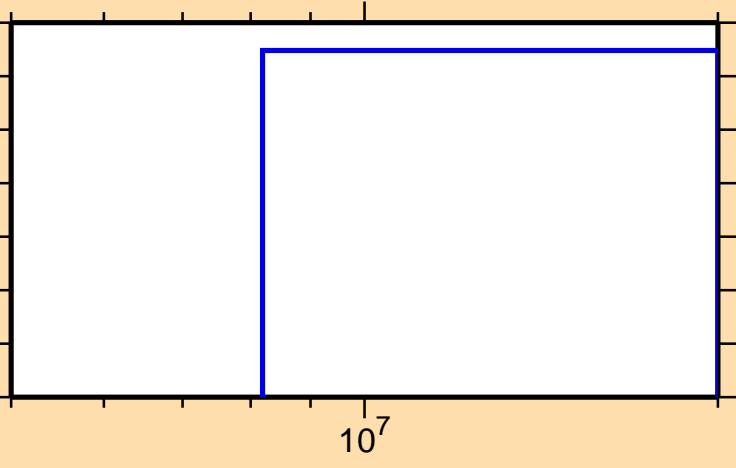
\sigma vs. E for ^{210}\text{Bi}(n,2np)
