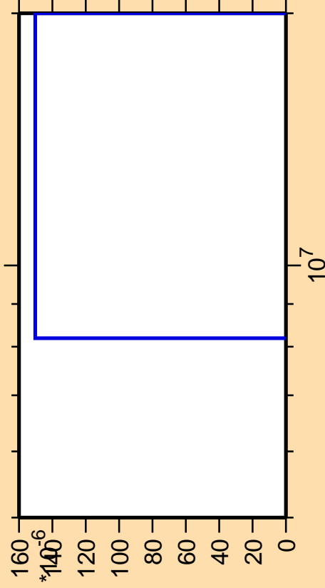
\Delta\sigma/\sigma vs. E for ^{210}\text{Bi}(n,\text{pt})
