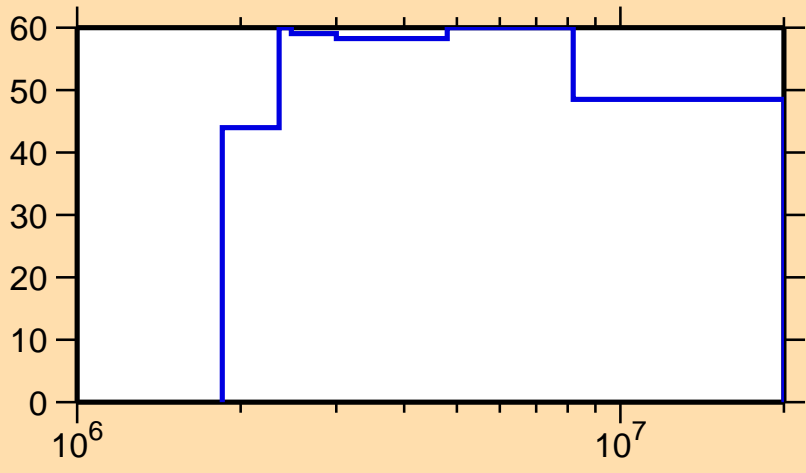
\Delta\sigma/\sigma vs. E for ^{210}\text{Bi}(n,p)
