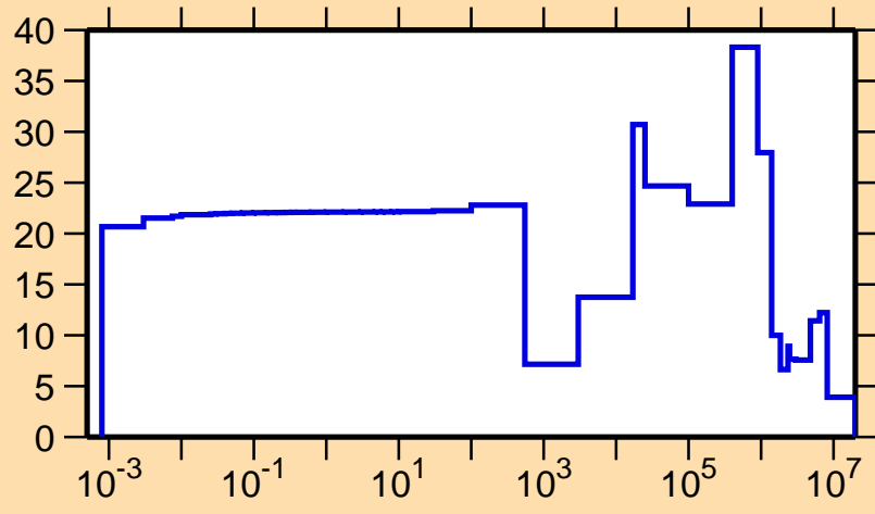
\Delta\sigma/\sigma vs. E for ^{210}\text{Bi}(n,\text{tot.})
