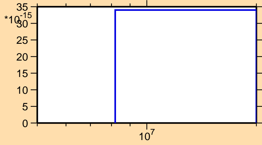
\sigma vs. E for ^{210}\text{Bi} (mt 45)
