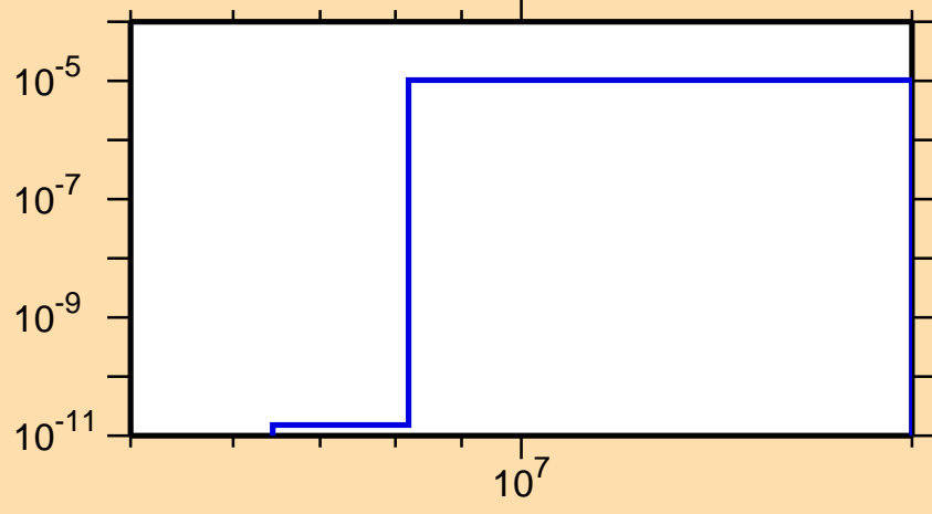
\sigma vs. E for ^{210}\text{Bi}(n,2n\alpha)
