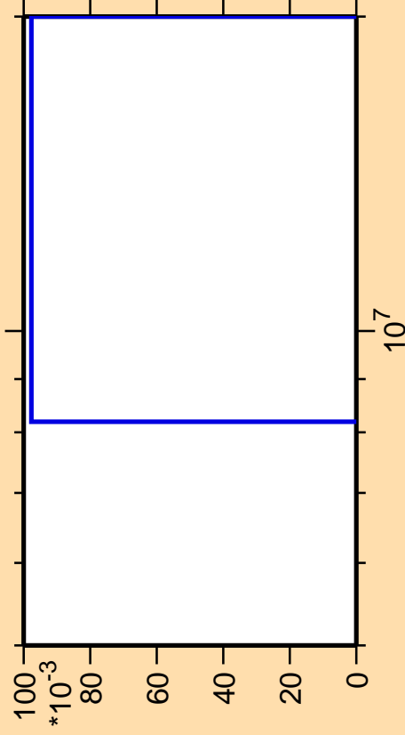
\Delta\sigma/\sigma vs. E for ^{210}\text{Bi} (mt 45)
