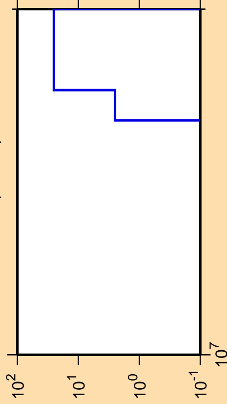
\Delta\sigma/\sigma vs. E for ^{210}\text{Bi} (mt 45)
