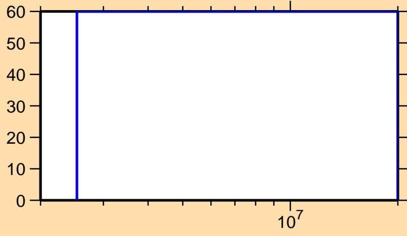
\Delta\sigma/\sigma vs. E for ^{210}\text{Bi}(n,\gamma)
