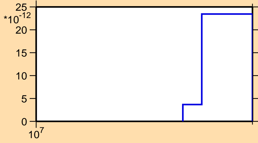
\sigma vs. E for ^{210}\text{Bi}(\text{mt117})
