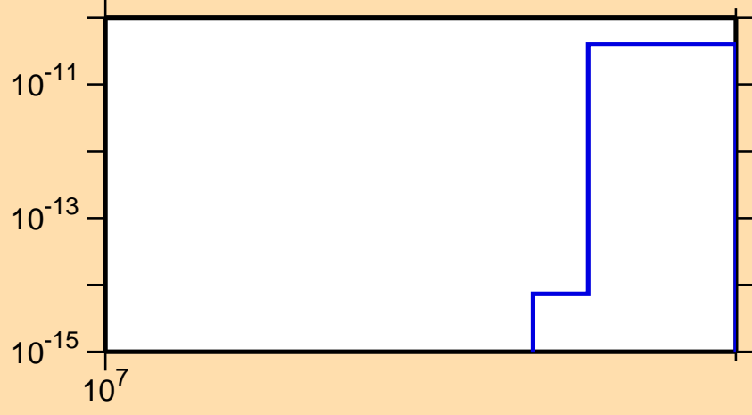
\sigma vs. E for ^{210}\text{Bi} (mt 42)
