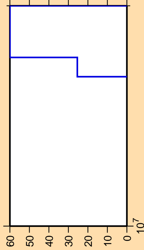
\Delta\sigma/\sigma vs. E for ^{210}\text{Bi}(\text{mt117})
