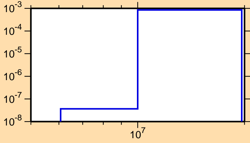
\sigma vs. E for ^{210}\text{Bi}(n,np)
