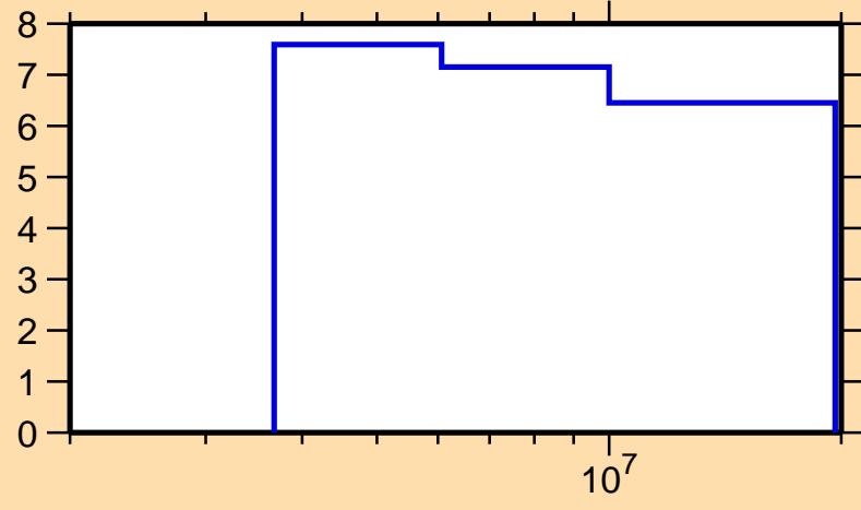
\Delta\sigma/\sigma vs. E for ^{210}\text{Bi}(n,\text{nonel.})
