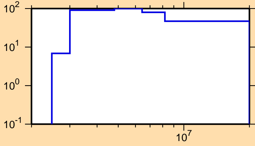
\Delta\sigma/\sigma vs. E for ^{210}\text{Bi}(n,p)
