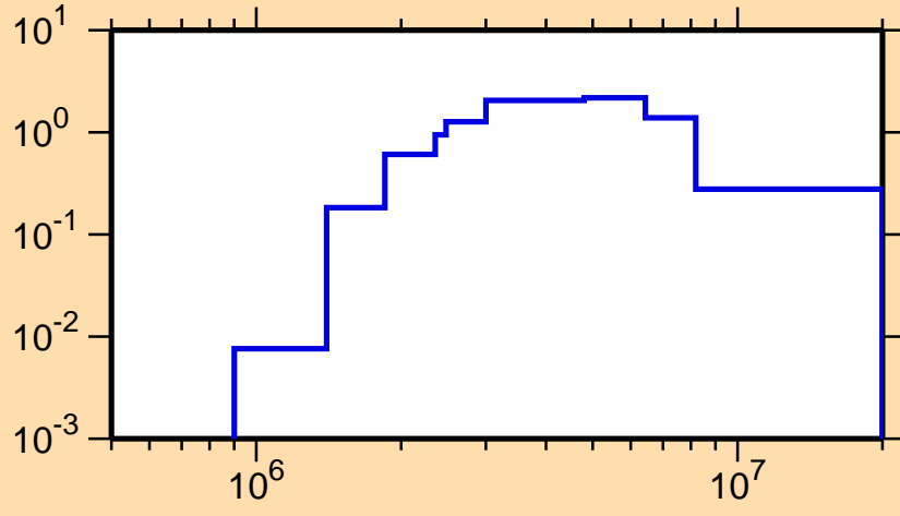
\sigma vs. E for ^{210}\text{Bi}(n,n\text{cont.})
