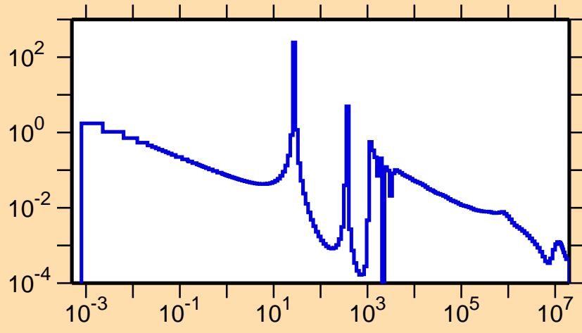
\sigma vs. E for ^{211}\text{Bi}(n,\gamma)
