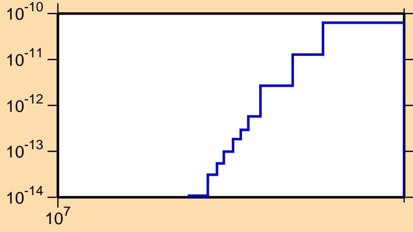
\sigma vs. E for ^{211}\text{Bi} (mt 45)
