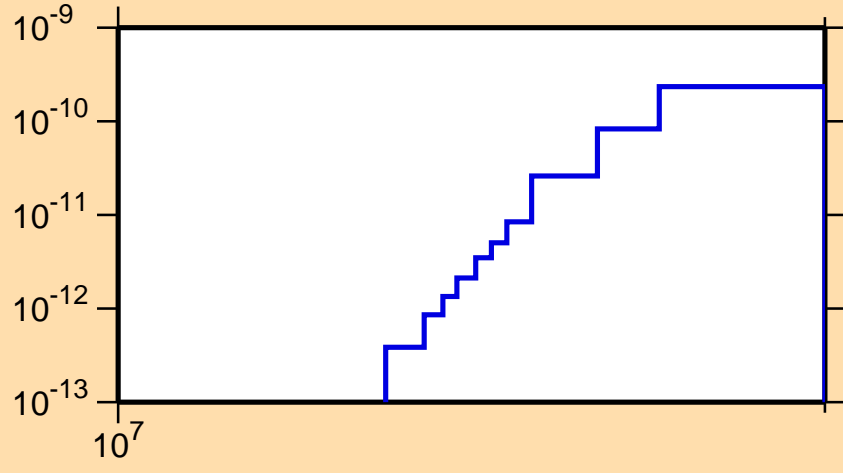
\sigma vs. E for ^{211}\text{Bi}(\text{mt117})
