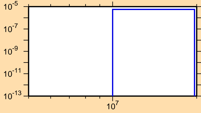
\sigma vs. E for ^{211}\text{Bi}(n,\text{nd})
