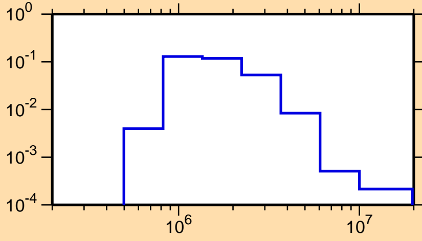
\sigma vs. E for ^{211}\text{Bi}(n,n_2)
