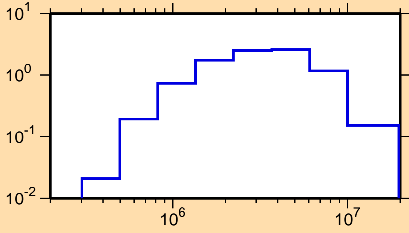
\sigma vs. E for ^{211}\text{Bi}(n,\text{inel.})
