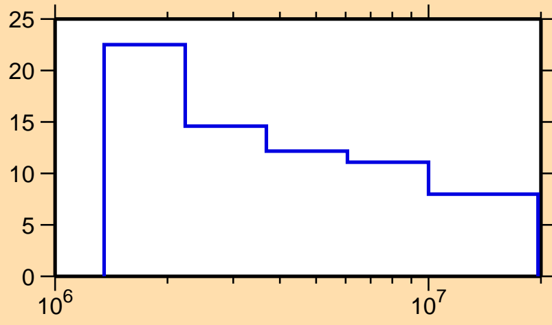
\Delta\sigma/\sigma vs. E for ^{212}\text{Bi}(n,n\text{nonel.})
