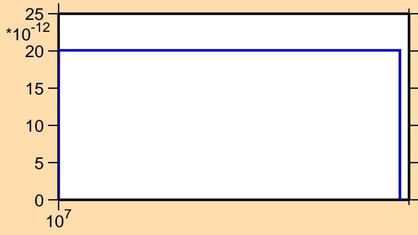
\sigma vs. E for ^{212}\text{Bi} (mt 42)
