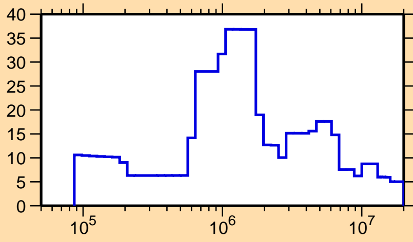
\Delta\sigma/\sigma vs. E for ^{212}\text{Bi}(n, el.)
