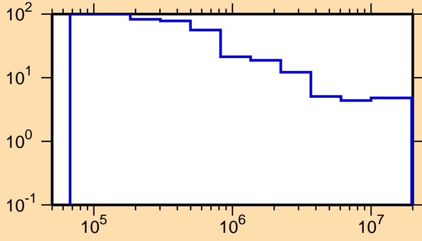
\Delta\sigma/\sigma vs. E for ^{212}\text{Bi}(n,n\text{nonel.})
