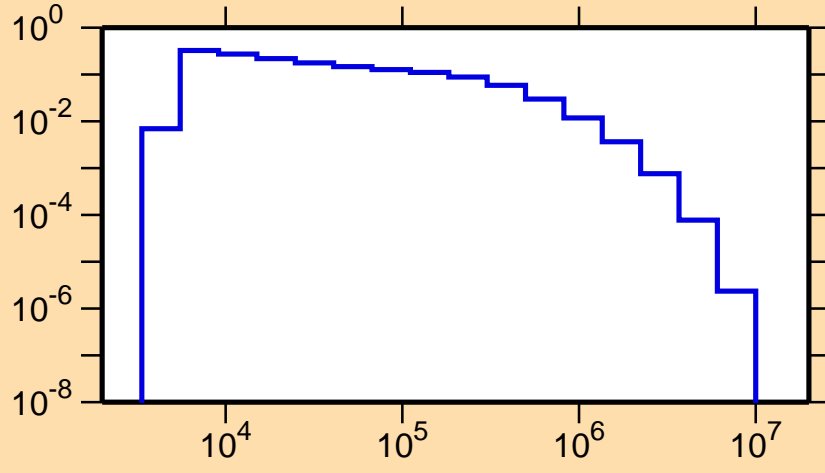
\sigma vs. E for ^{212}\text{Bi}(n,n_4)
