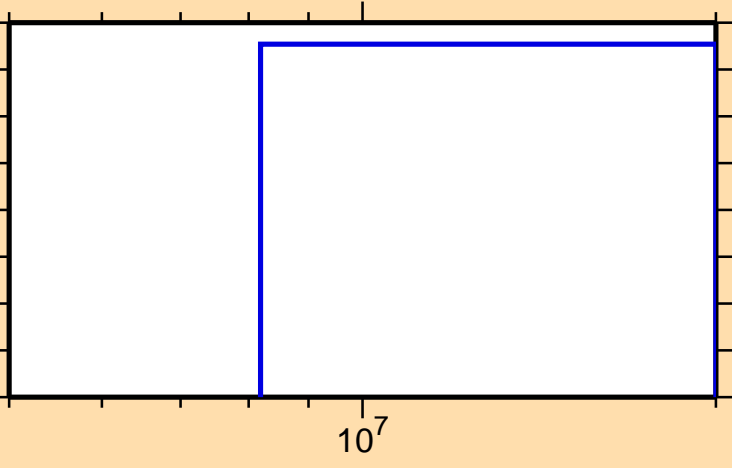
\sigma vs. E for ^{212}\text{Bi} (mt 34)
