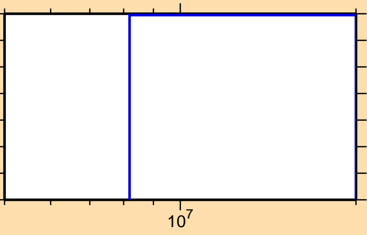
\sigma vs. E for ^{212}\text{Bi}(\text{mt117})
