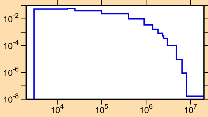
\sigma vs. E for ^{212}\text{Bi}(n,n_1)
