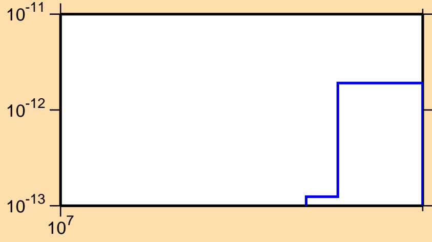
\sigma vs. E for ^{213}\text{Bi} (mt 45)
