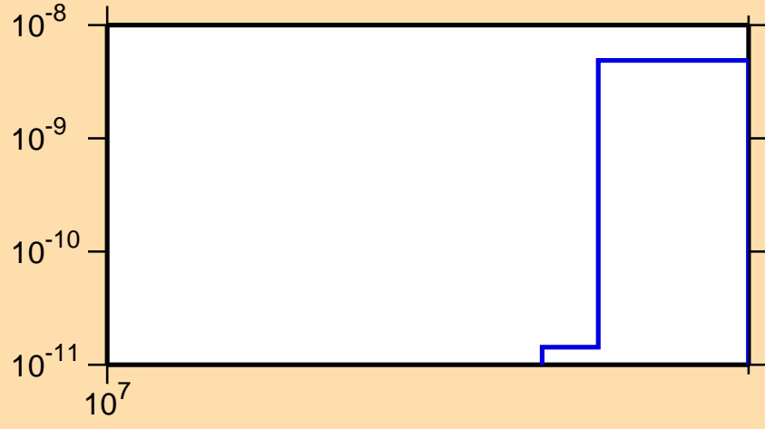
\sigma vs. E for ^{213}\text{Bi} (mt 11)
