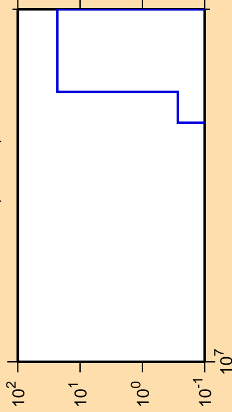
\Delta\sigma/\sigma vs. E for ^{213}\text{Bi}(n,\text{He}3)
