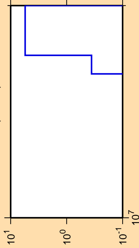
\Delta\sigma/\sigma vs. E for ^{213}\text{Bi} (mt 45)
