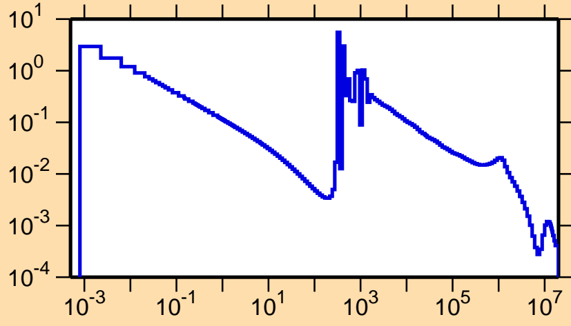
\sigma vs. E for ^{213}\text{Bi}(n,\gamma)
