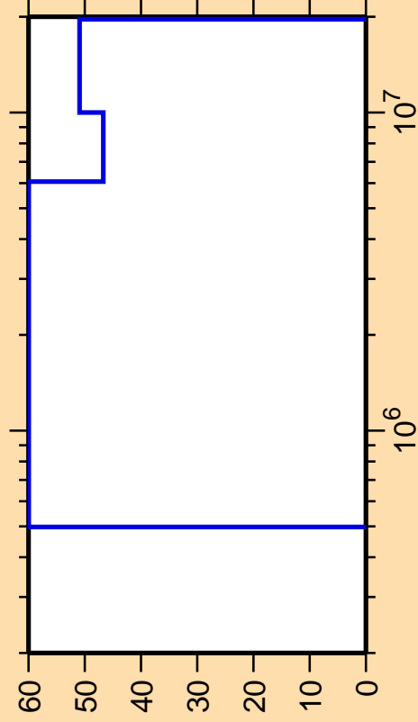
\Delta\sigma/\sigma vs. E for ^{213}\text{Bi}(n,n_2)
