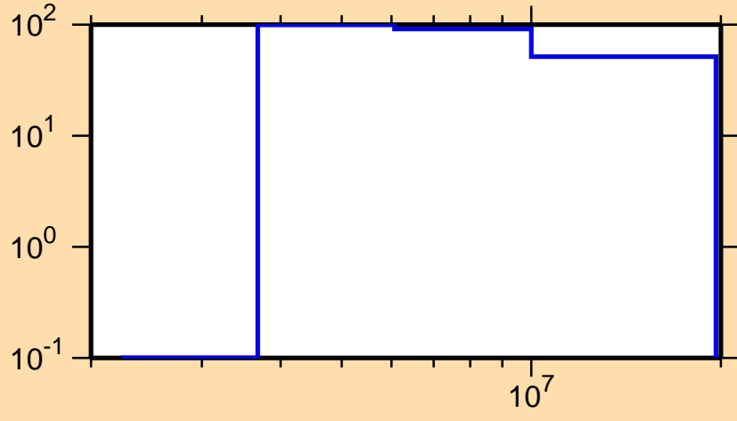
\Delta\sigma/\sigma vs. E for ^{213}\text{Bi}(n,p)
