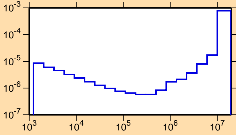
\sigma vs. E for ^{213}\text{Bi}(n,\alpha)
