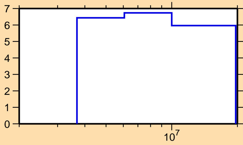
\Delta\sigma/\sigma vs. E for ^{213}\text{Bi}(n,\text{tot.})
