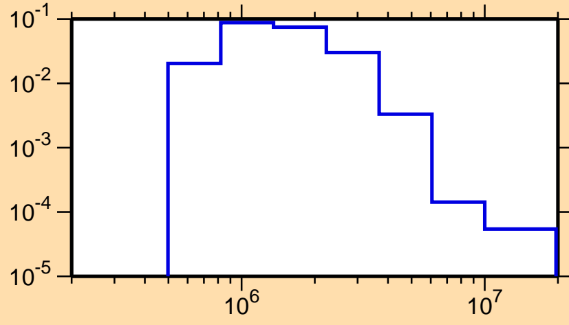
\sigma vs. E for ^{213}\text{Bi}(n,n_2)
