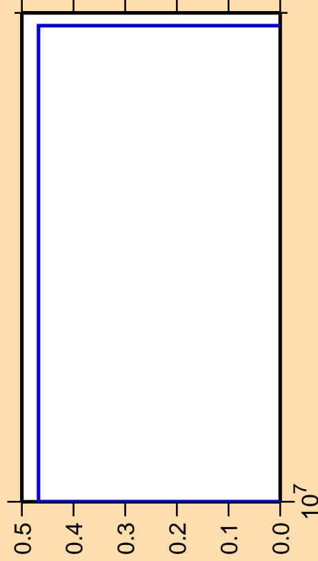
\Delta\sigma/\sigma vs. E for ^{213}\text{Bi}(\text{mt117})
