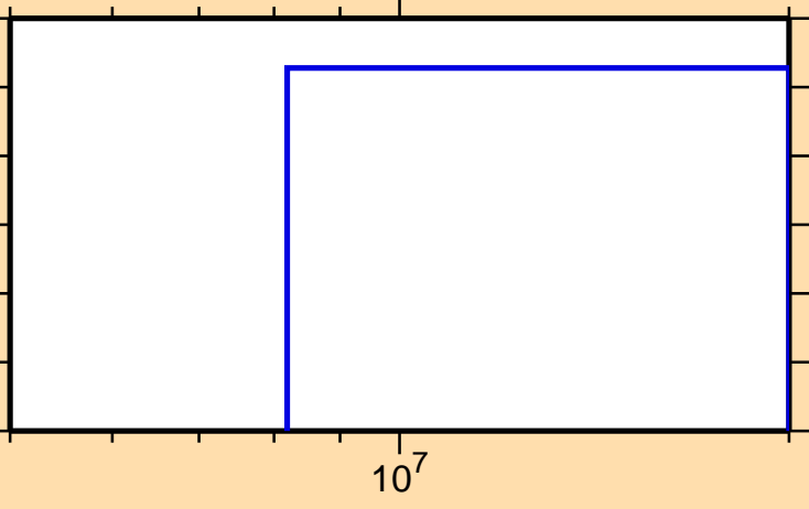
\sigma vs. E for ^{213}\text{Bi}(n,2np)
