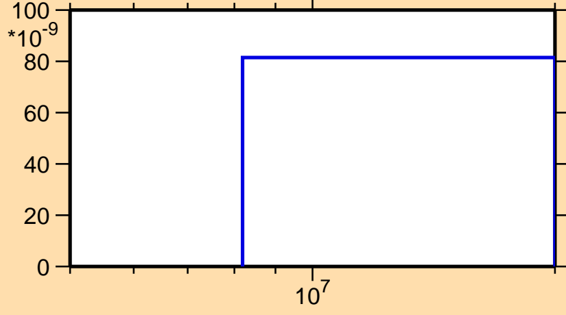
\sigma vs. E for ^{213}\text{Bi}(n,p\alpha)
