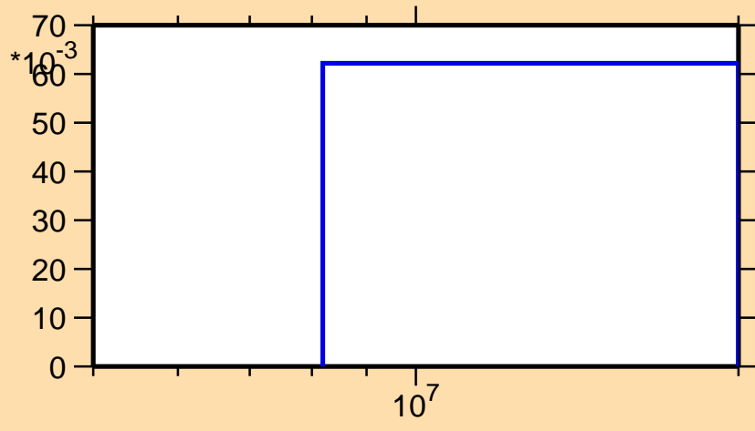
\sigma vs. E for ^{213}\text{Bi}(n,3n\alpha)
