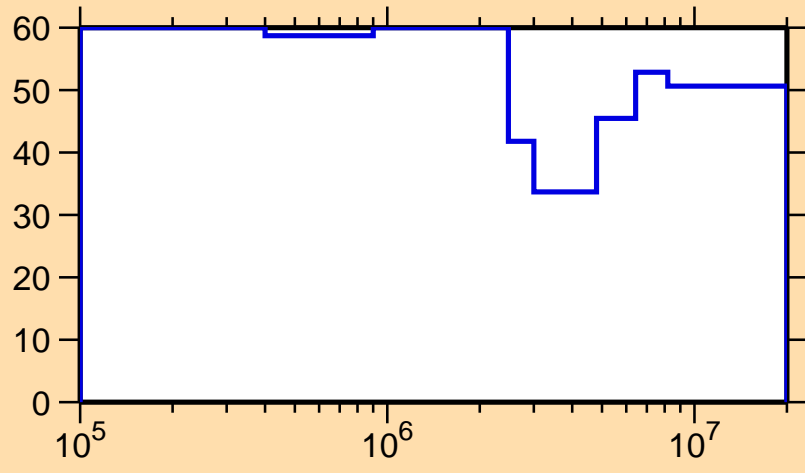
\Delta\sigma/\sigma vs. E for ^{213}\text{Bi}(n,n_1)
