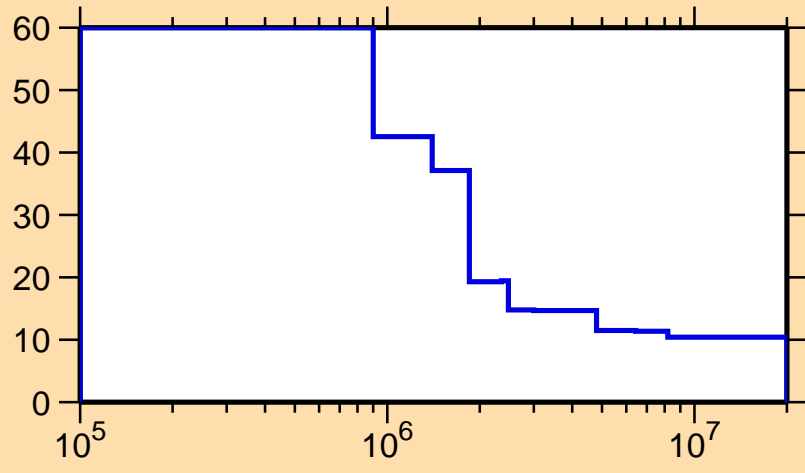
\Delta\sigma/\sigma vs. E for ^{213}\text{Bi}(n,\text{nonel.})
