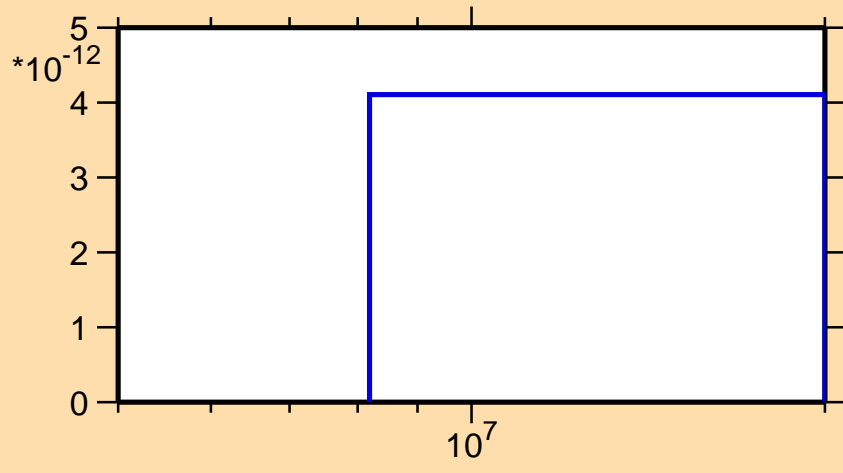
\sigma vs. E for ^{213}\text{Bi} (mt 42)
