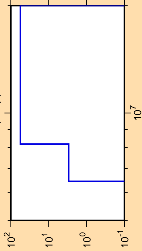
\Delta\sigma/\sigma vs. E for ^{213}\text{Bi}(n,np)
