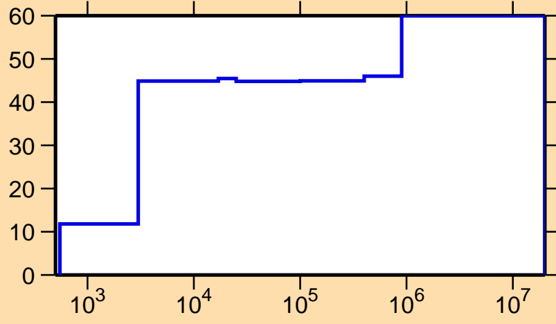
\Delta\sigma/\sigma vs. E for ^{213}\text{Bi}(n,\gamma)
