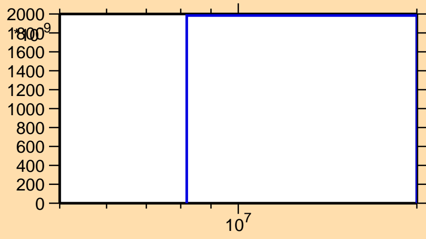
\sigma vs. E for ^{213}\text{Bi}(n,\text{nd})
