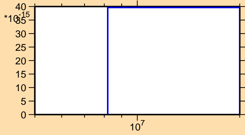
\sigma vs. E for ^{213}\text{Bi}(n,\text{He3})
