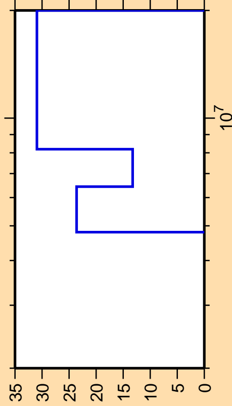
\Delta\sigma/\sigma vs. E for ^{213}\text{Bi}(n,2n)
