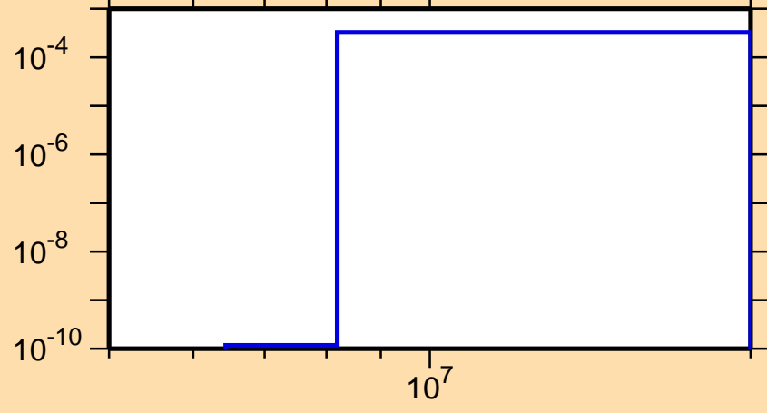
\sigma vs. E for ^{213}\text{Bi}(n,d)
