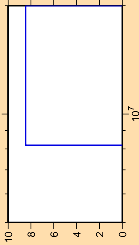
\Delta\sigma/\sigma vs. E for ^{213}\text{Bi} (mt 42)
