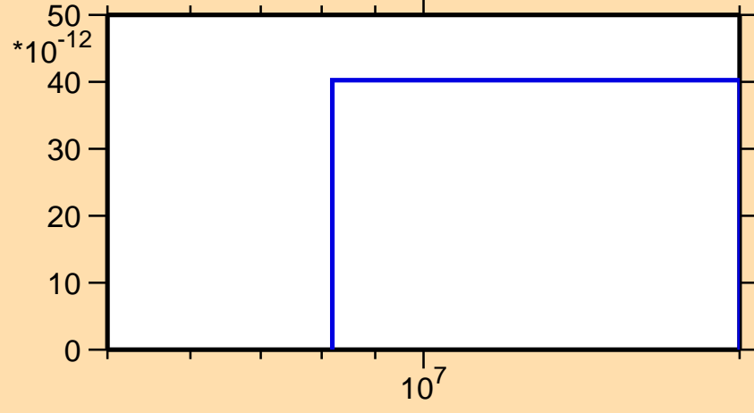
\sigma vs. E for ^{213}\text{Bi} (mt 11)
