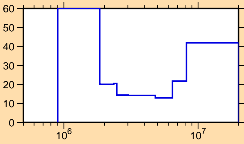
\Delta\sigma/\sigma vs. E for ^{213}\text{Bi}(n,n\text{cont.})
