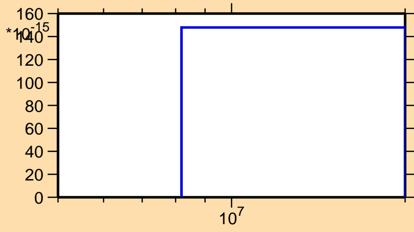
\sigma vs. E for ^{213}\text{Bi}(\text{mt117})
