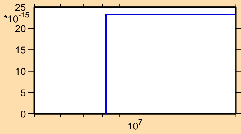
\sigma vs. E for ^{213}\text{Bi} (mt 45)
