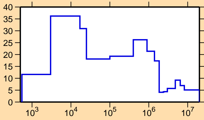
\Delta\sigma/\sigma vs. E for ^{213}\text{Bi}(n,\text{tot.})
