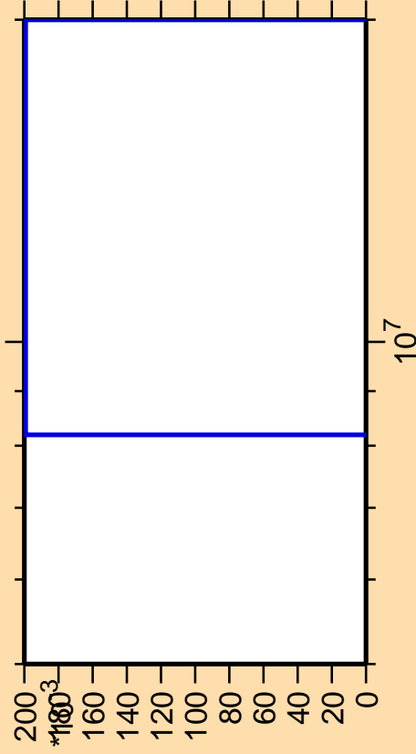
\Delta\sigma/\sigma vs. E for ^{213}\text{Bi}(n,\text{He3})
