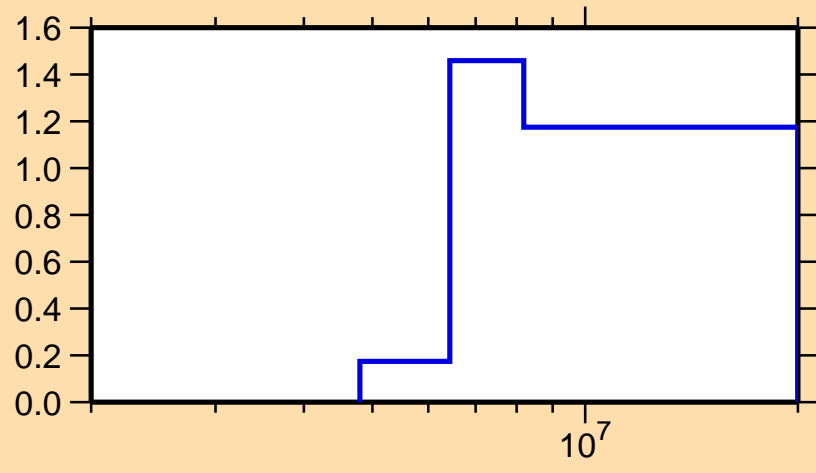
\sigma vs. E for ^{213}\text{Bi}(n,2n)
