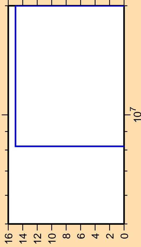
\Delta\sigma/\sigma vs. E for ^{213}\text{Bi}(n,3n)
