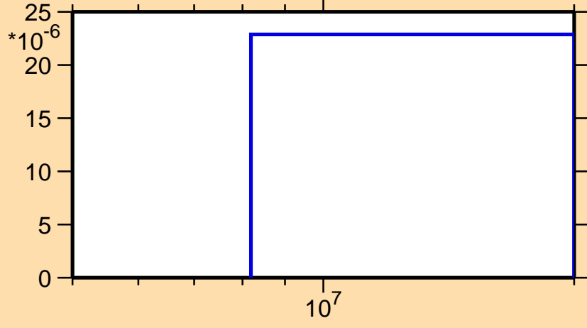
\sigma vs. E for ^{213}\text{Bi}(n,nt)
