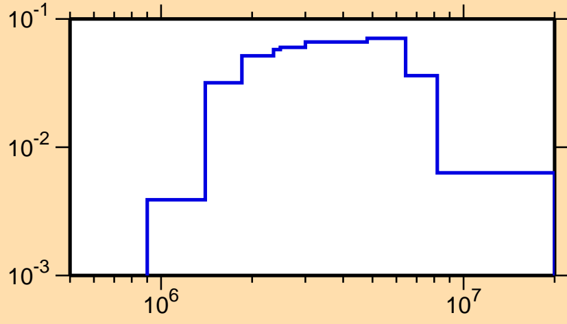
\sigma vs. E for ^{213}\text{Bi}(n,n\alpha)
