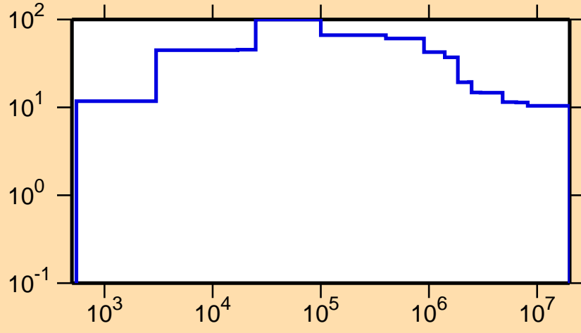
\Delta\sigma/\sigma vs. E for ^{213}\text{Bi}(n,\text{nonel.})
