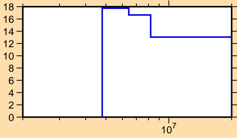
\Delta\sigma/\sigma vs. E for ^{213}\text{Bi}(n,\text{el.})
