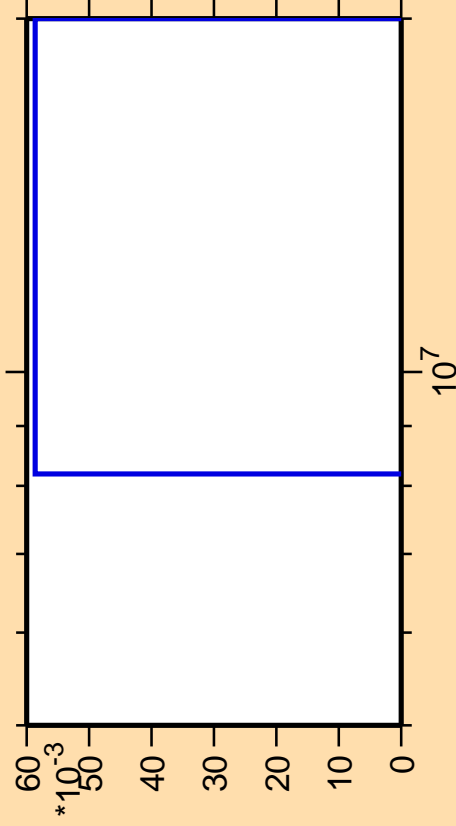
\Delta\sigma/\sigma vs. E for ^{213}\text{Bi} (mt 45)
