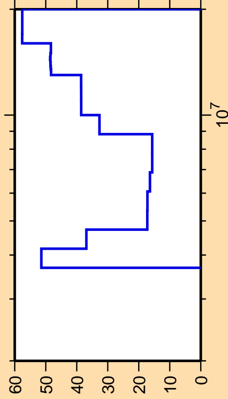
\Delta\sigma/\sigma vs. E for ^{214}\text{Bi}(n,2n)
