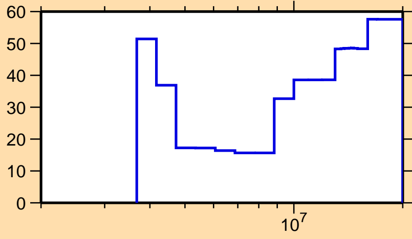
\Delta\sigma/\sigma vs. E for ^{214}\text{Bi}(n,2n)
