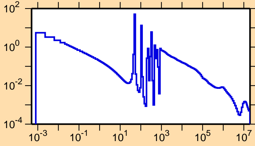
\sigma vs. E for ^{214}\text{Bi}(n,\gamma)
