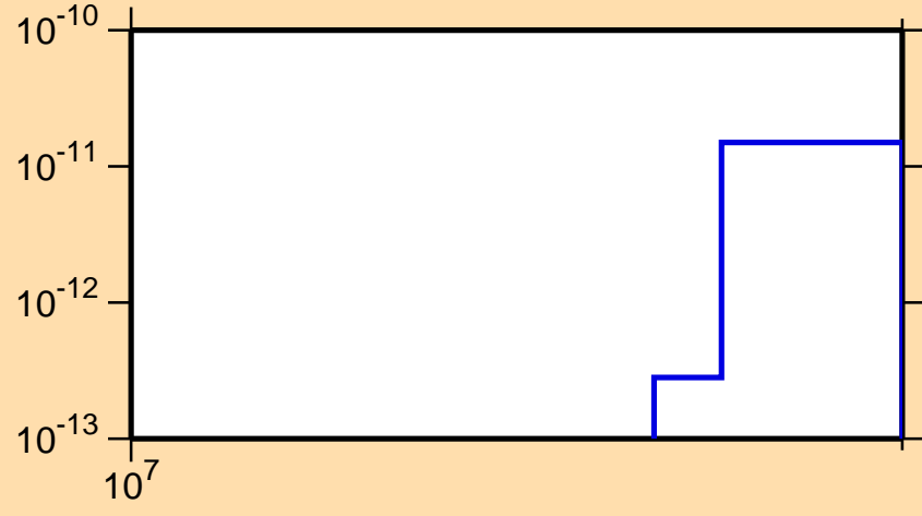
\sigma vs. E for ^{214}\text{Bi}(n,\text{He}3)
