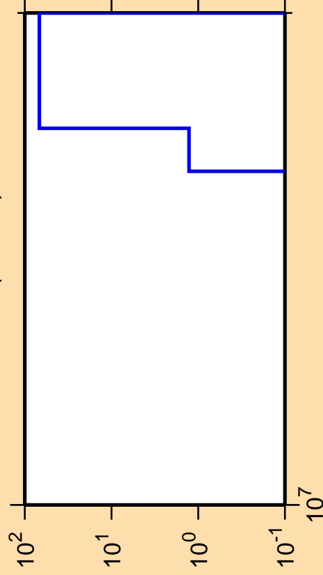
\Delta\sigma/\sigma vs. E for ^{214}\text{Bi}(n,\text{He}3)
