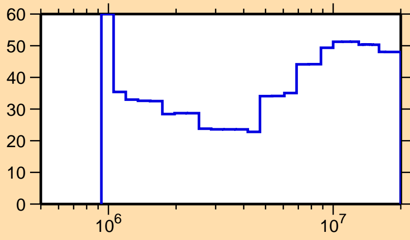
\Delta\sigma/\sigma vs. E for ^{214}\text{Bi}(n,n\text{cont.})
