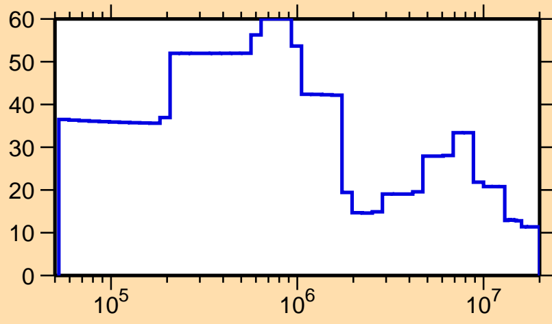
\Delta\sigma/\sigma vs. E for ^{214}\text{Bi}(n,\text{el.})
