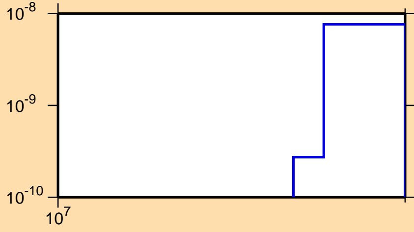
\sigma vs. E for ^{214}\text{Bi} (mt 45)
