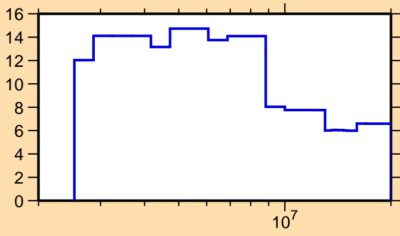
\Delta\sigma/\sigma vs. E for ^{214}\text{Bi}(n,\text{tot.})
