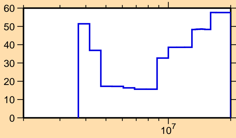
\Delta\sigma/\sigma vs. E for ^{214}\text{Bi}(n,2n)
