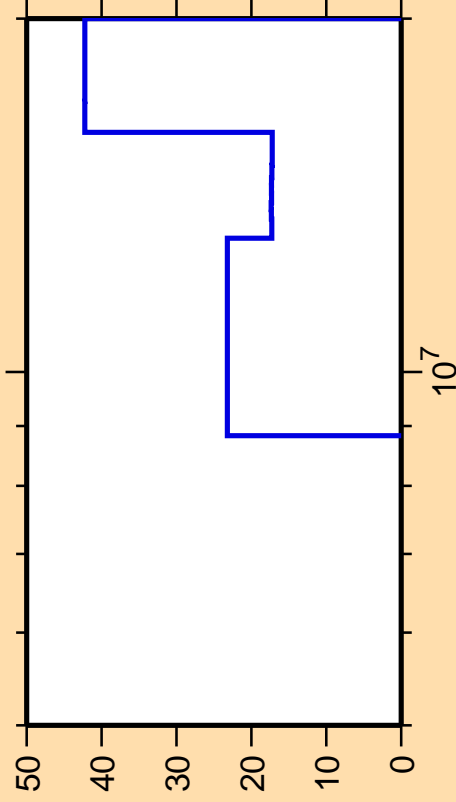
\Delta\sigma/\sigma vs. E for ^{214}\text{Bi}(n,3n)
