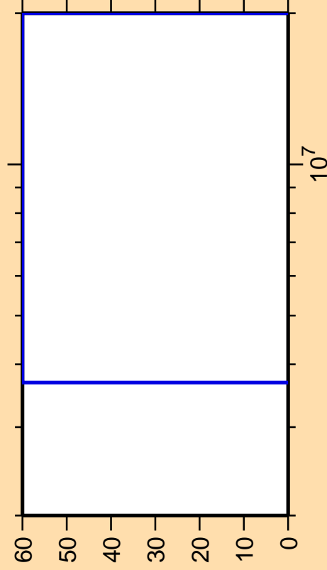
\Delta\sigma/\sigma vs. E for ^{214}\text{Bi}(n,p)
