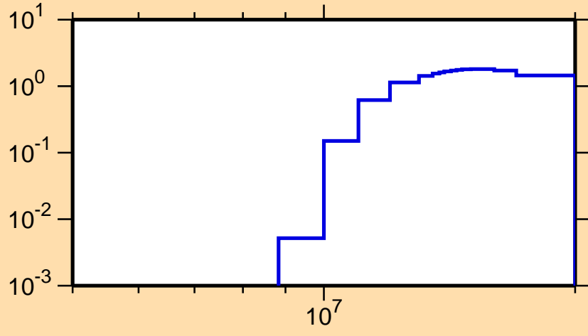
\sigma vs. E for ^{214}\text{Bi}(n,3n)
