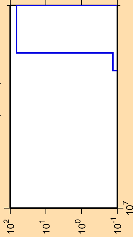
\Delta\sigma/\sigma vs. E for ^{214}\text{Bi} (mt 42)
