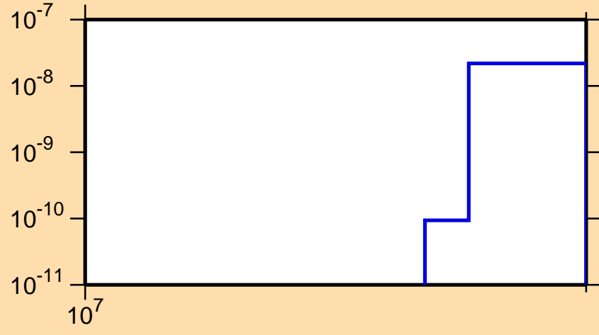
\sigma vs. E for ^{214}\text{Bi} (mt 11)
