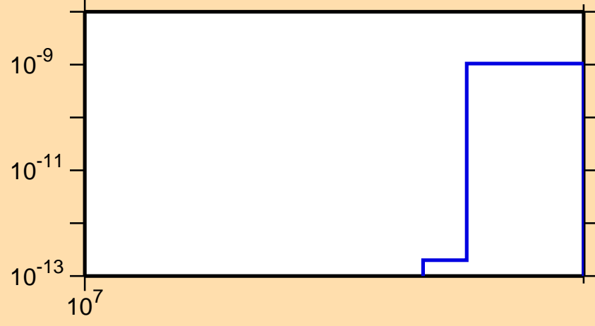
\sigma vs. E for ^{214}\text{Bi} (mt 42)
