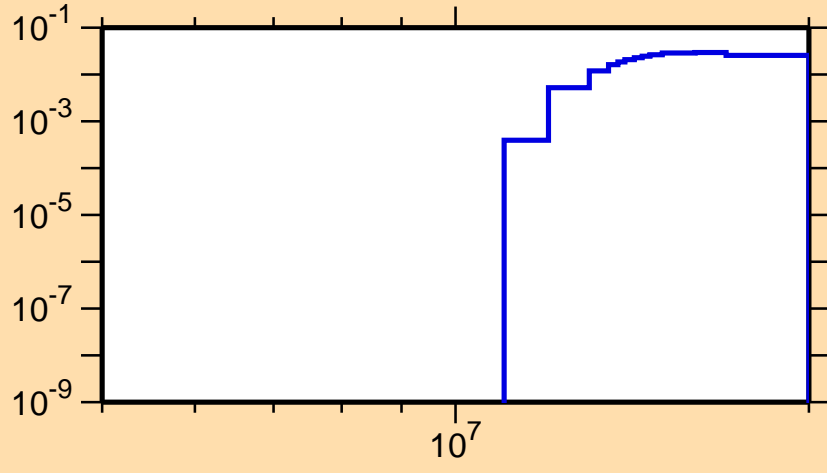
\sigma vs. E for ^{214}\text{Bi}(n,3n\alpha)
