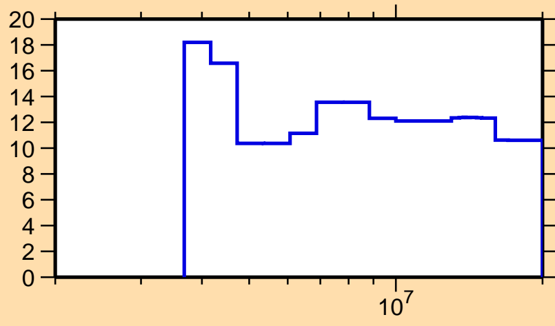
\Delta\sigma/\sigma vs. E for ^{214}\text{Bi}(n,\text{nonel.})
