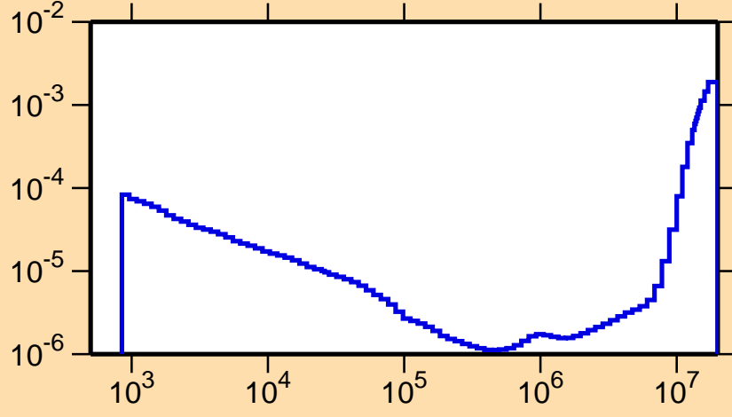
\sigma vs. E for ^{214}\text{Bi}(n,\alpha)
