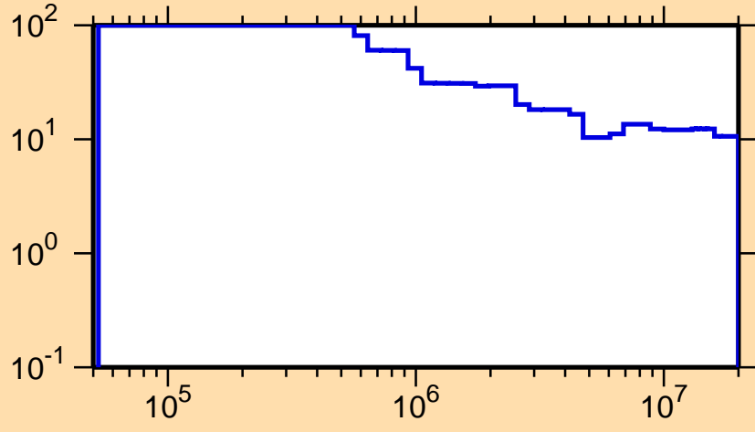
\Delta\sigma/\sigma vs. E for ^{214}\text{Bi}(n,\text{nonel.})
