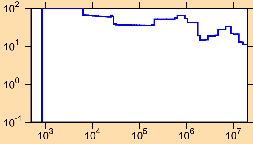
\Delta\sigma/\sigma vs. E for ^{214}\text{Bi}(n,\text{el.})
