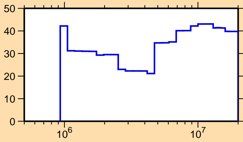
\Delta\sigma/\sigma vs. E for ^{214}\text{Bi}(n,\text{inel.})
