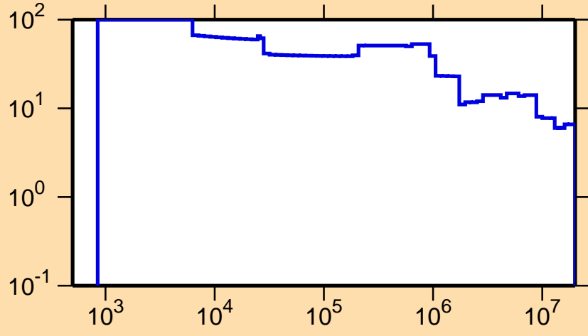
\Delta\sigma/\sigma vs. E for ^{214}\text{Bi}(n,\text{tot.})
