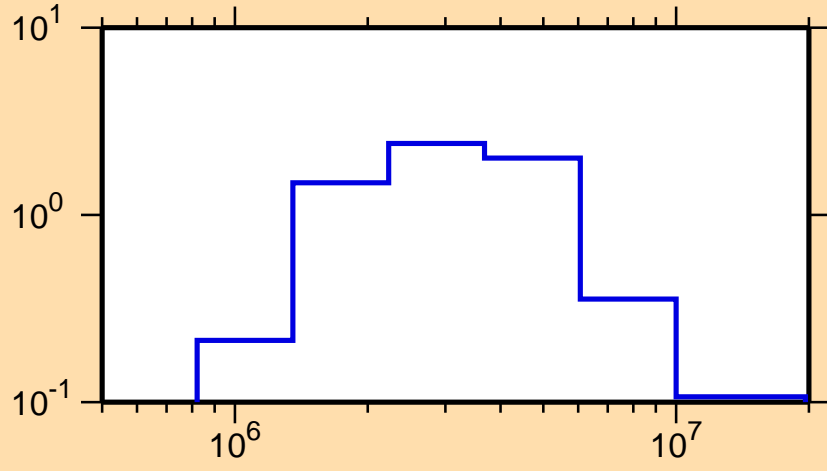
\sigma vs. E for ^{214}\text{Bi}(n,n\text{cont.})
