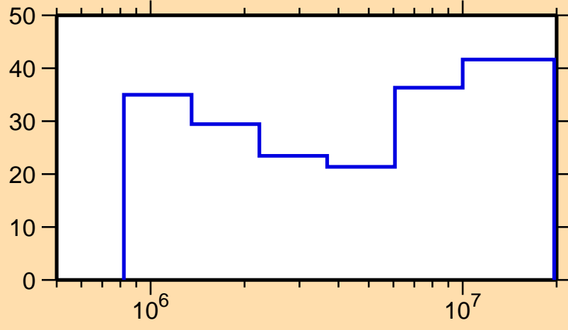
\Delta\sigma/\sigma vs. E for ^{214}\text{Bi}(n,\text{inel.})
