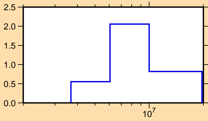
\sigma vs. E for ^{214}\text{Bi}(n,2n)
