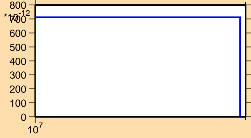
\sigma vs. E for ^{214}\text{Bi}(\text{mt117})
