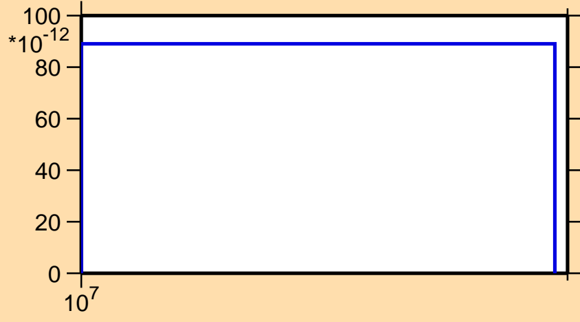
\sigma vs. E for ^{214}\text{Bi} (mt 45)
