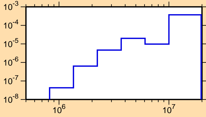
\sigma vs. E for ^{214}\text{Bi}(n,n\alpha)
