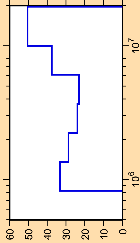
\Delta\sigma/\sigma vs. E for ^{214}\text{Bi}(n,n\text{cont.})
