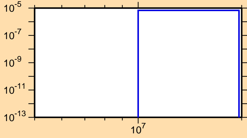
\sigma vs. E for ^{214}\text{Bi}(n,\text{nd})
