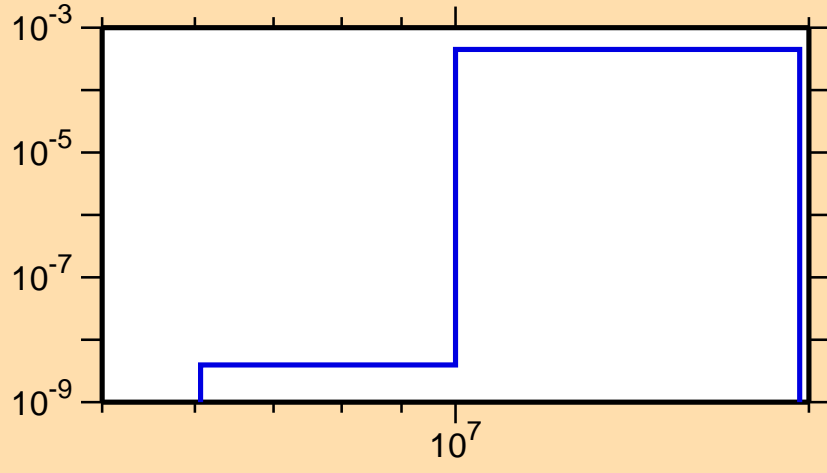
\sigma vs. E for ^{214}\text{Bi}(n,d)
