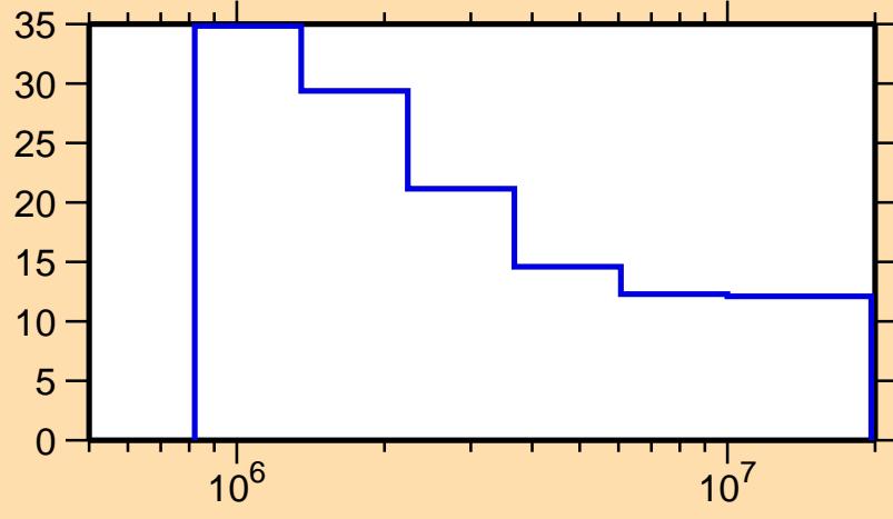
\Delta\sigma/\sigma vs. E for ^{214}\text{Bi}(n,n\text{nonel.})
