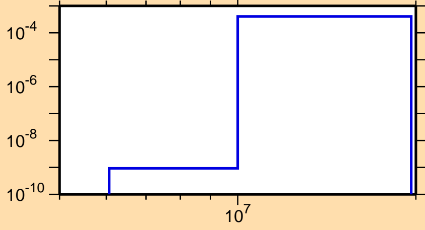
\sigma vs. E for ^{214}\text{Bi}(n,np)
