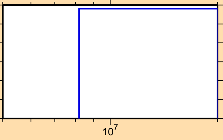
\sigma vs. E for ^{214}\text{Bi}(\text{mt117})
