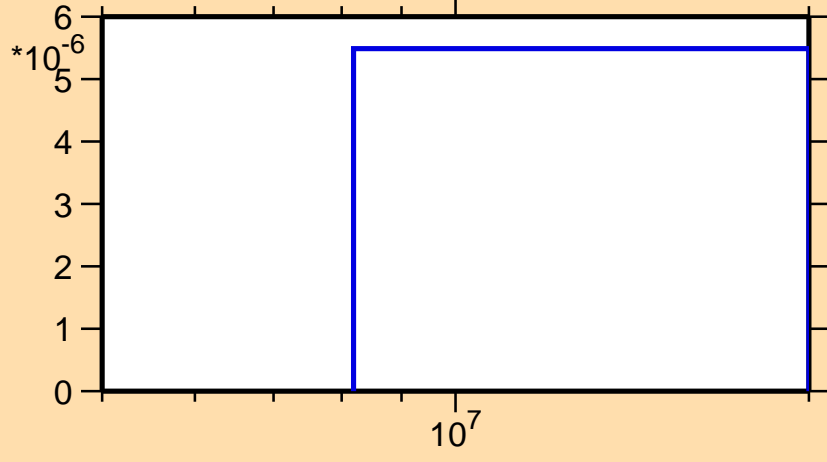
\sigma vs. E for ^{214}\text{Bi}(n,\text{nd})
