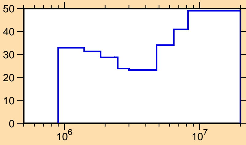
\Delta\sigma/\sigma vs. E for ^{214}\text{Bi}(n,ncont.)
