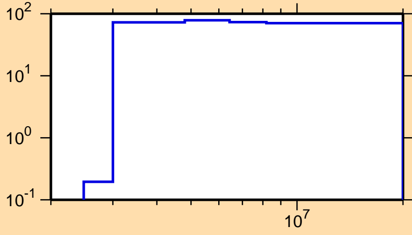
\Delta\sigma/\sigma vs. E for ^{214}\text{Bi}(n,p)
