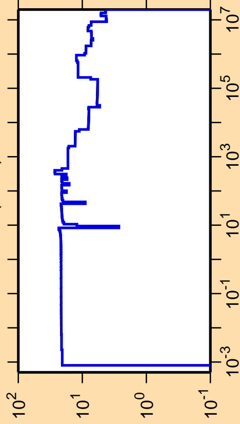
\Delta\sigma/\sigma vs. E for ^{215}\text{Bi}(n,\text{el.})
