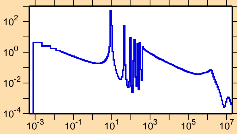
\sigma vs. E for ^{215}\text{Bi}(n,\gamma)
