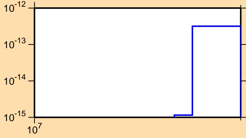
\sigma vs. E for ^{215}\text{Bi}(n,\text{He3})
