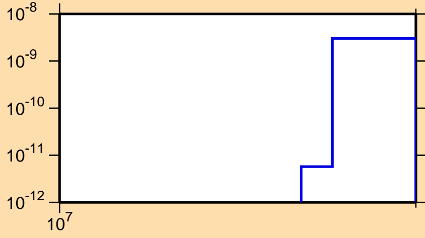
\sigma vs. E for ^{215}\text{Bi} (mt 11)
