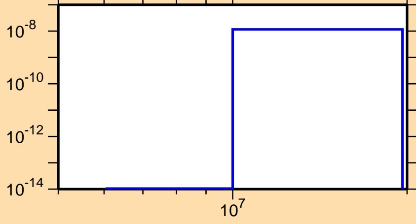
\sigma vs. E for ^{215}\text{Bi}(n,p\alpha)
