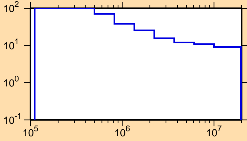
\Delta\sigma/\sigma vs. E for ^{215}\text{Bi}(n,n\text{nonel.})
