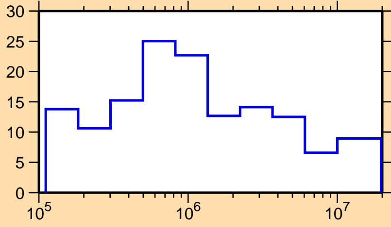
\Delta\sigma/\sigma vs. E for ^{215}\text{Bi}(n, tot.)
