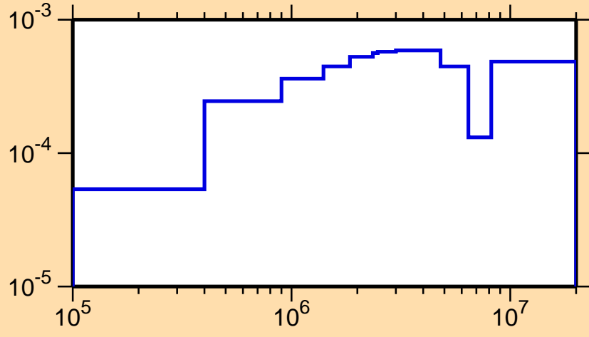
\sigma vs. E for ^{215}\text{Bi}(n,n\alpha)
