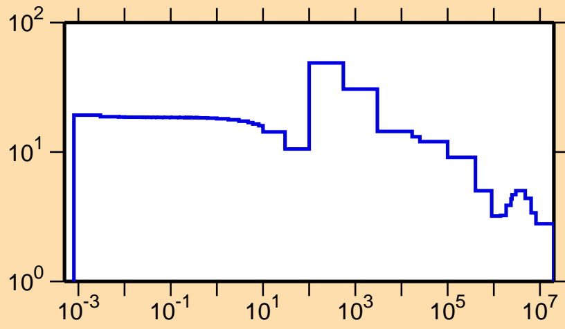
\sigma vs. E for ^{215}\text{Bi}(n,\text{el.})
