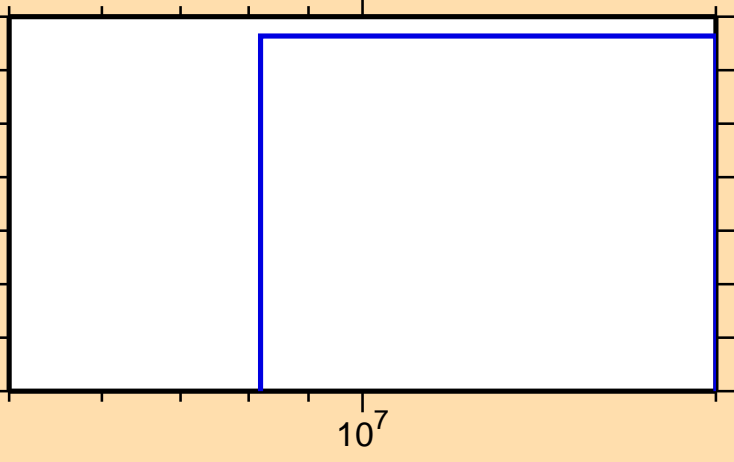
\sigma vs. E for ^{215}\text{Bi}(n,\text{nd})
