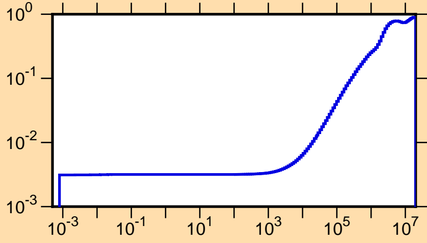
\mu vs. E for ^{216}\text{Bi}(\text{mt251})
