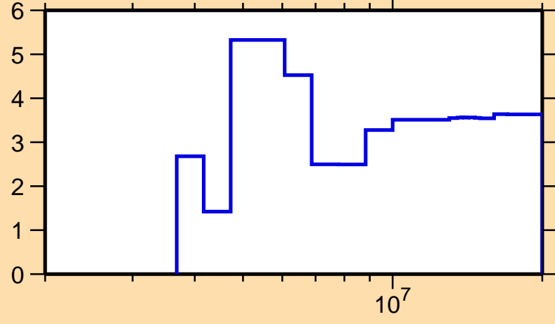
\Delta\sigma/\sigma vs. E for ^{216}\text{Bi}(n,\text{nonel.})
