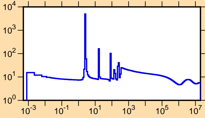
\sigma vs. E for ^{216}\text{Bi}(n,\text{tot.})
