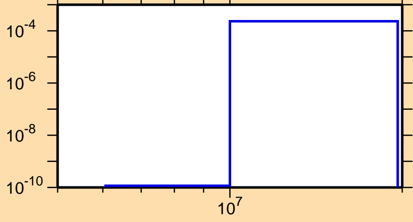
\sigma vs. E for ^{216}\text{Bi}(n,np)
