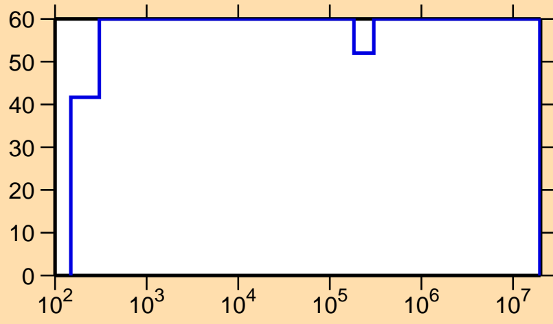
\Delta\sigma/\sigma vs. E for ^{216}\text{Bi}(n,\gamma)
