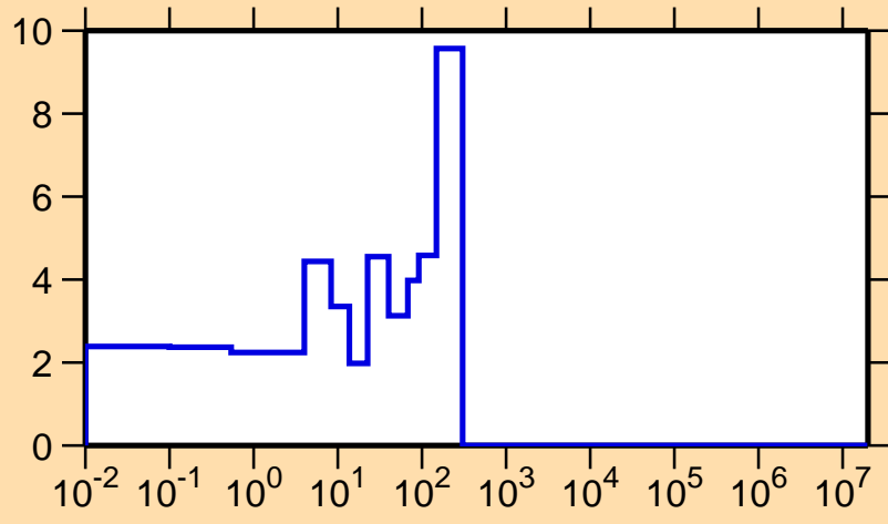
\Delta\sigma/\sigma vs. E for ^{216}\text{Bi}(n,f)
