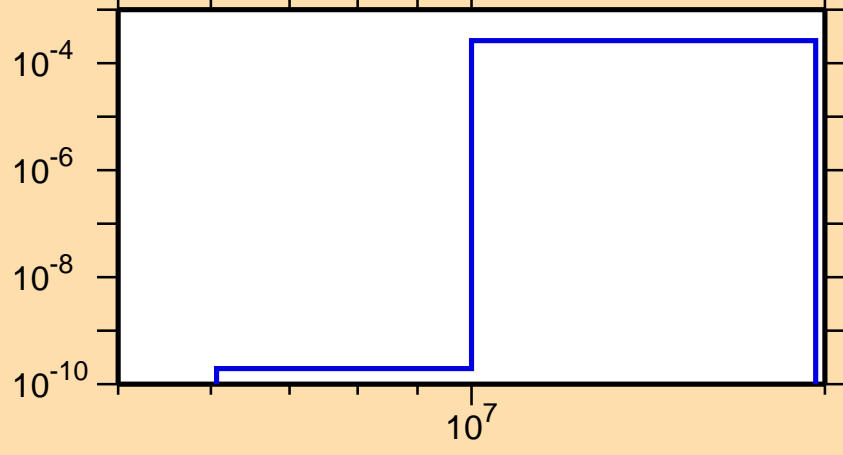
\sigma vs. E for ^{216}\text{Bi}(n,np)
