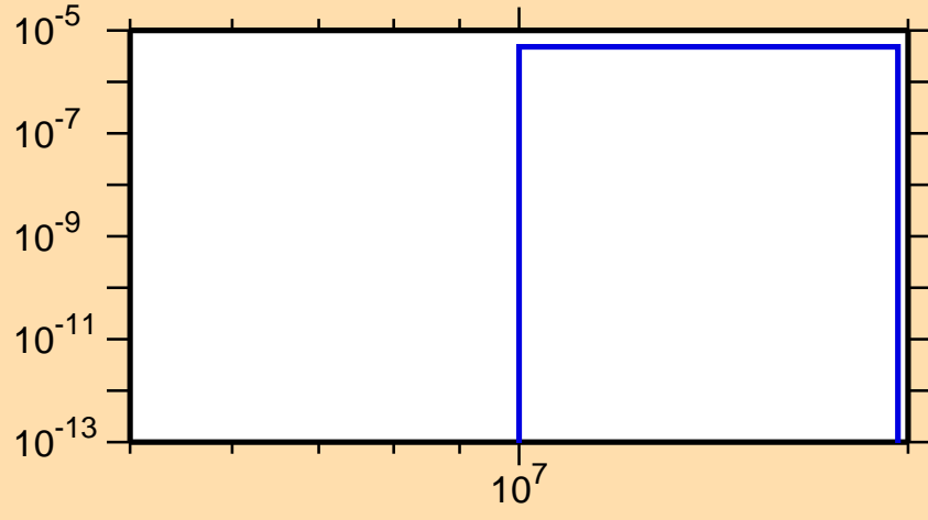
\sigma vs. E for ^{216}\text{Bi}(n,nd)
