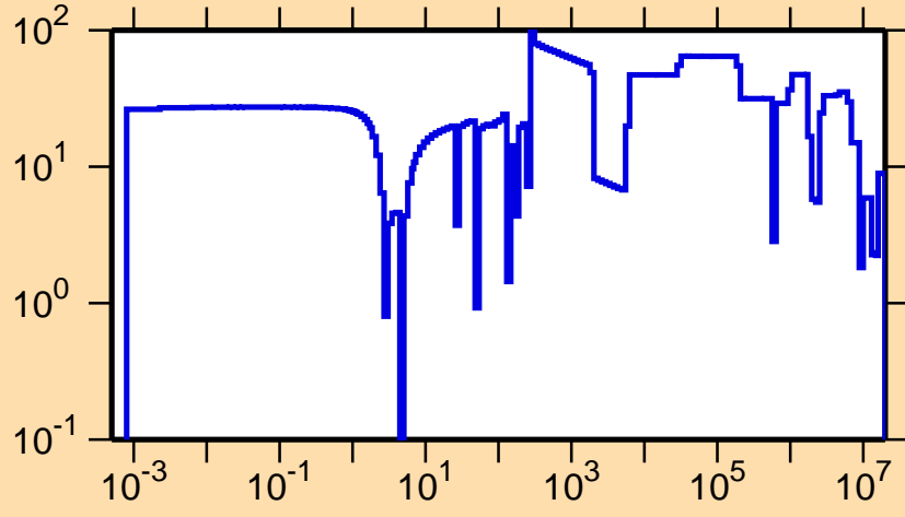
\Delta\sigma/\sigma vs. E for ^{217}\text{Bi}(n,el.)
