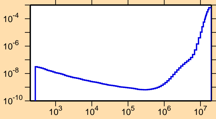
\sigma vs. E for ^{217}\text{Bi}(n,\alpha)
