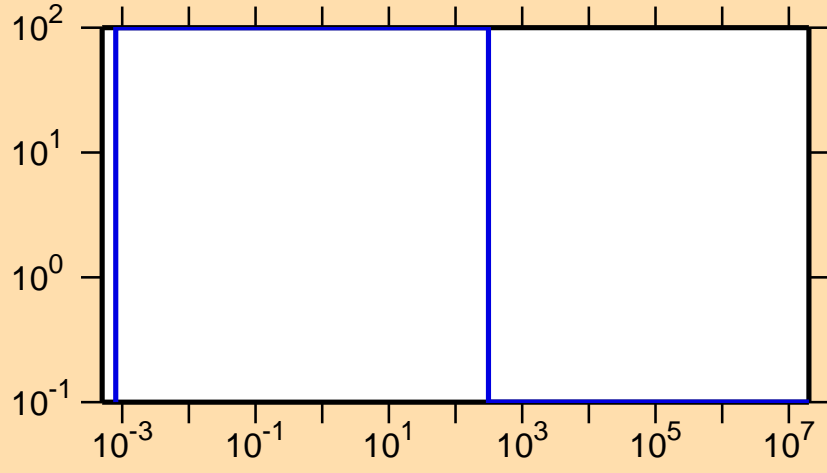
\Delta\sigma/\sigma vs. E for ^{217}\text{Bi}(n,f)
