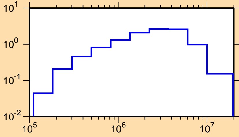
\sigma vs. E for ^{217}\text{Bi}(n,\text{inel.})
