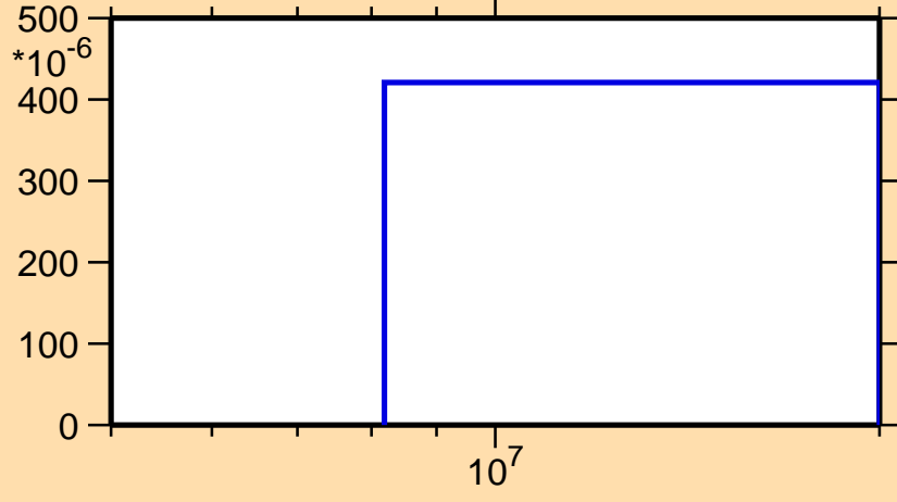
\sigma vs. E for ^{217}\text{Bi}(n,3n\alpha)
