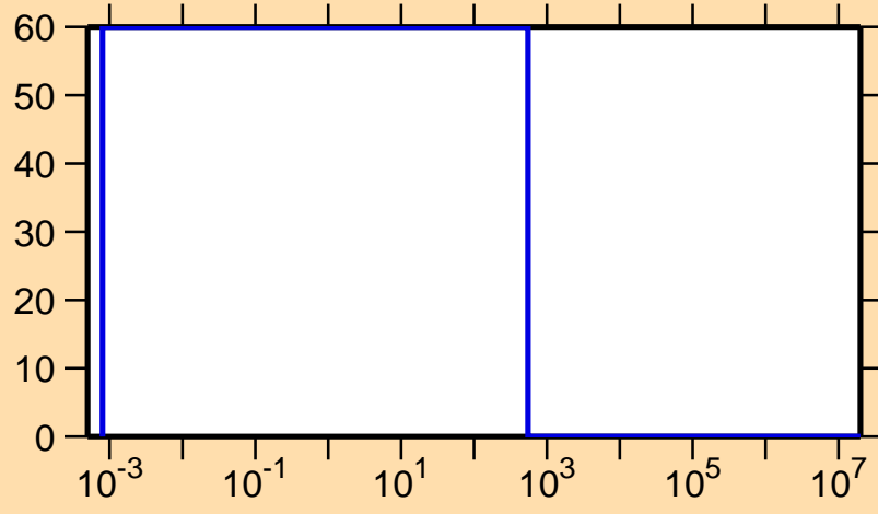
\Delta\sigma/\sigma vs. E for ^{217}\text{Bi}(n,f)
