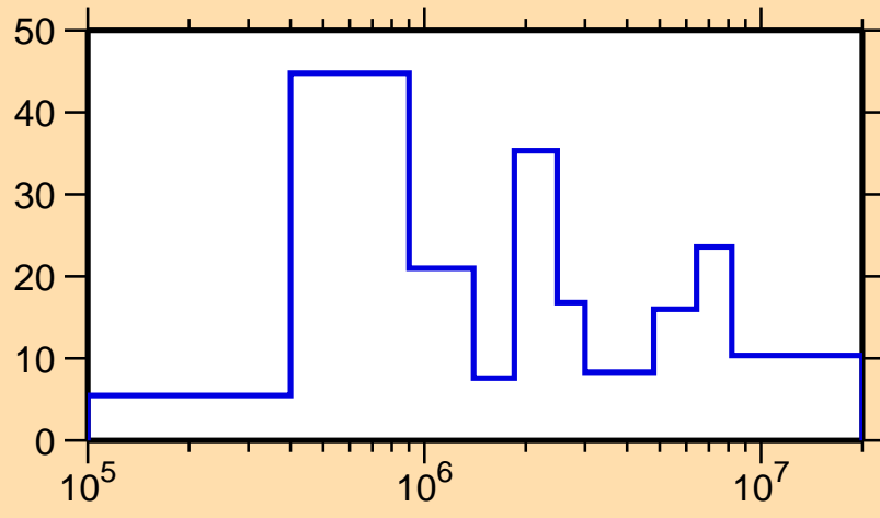
\Delta\sigma/\sigma vs. E for ^{217}\text{Bi}(n,n_1)
