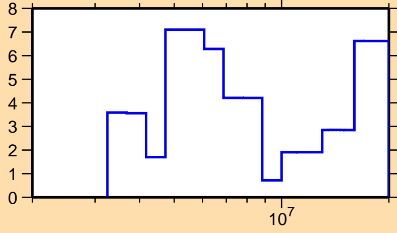
\Delta\sigma/\sigma vs. E for ^{218}\text{Bi}(n,\text{nonel.})
