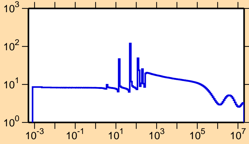
\sigma vs. E for ^{218}\text{Bi}(n,\text{el.})
