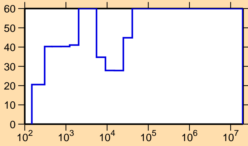
\Delta\sigma/\sigma vs. E for ^{218}\text{Bi}(n,\gamma)
