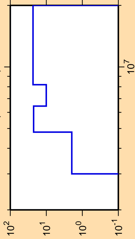
\Delta\sigma/\sigma vs. E for ^{218}\text{Bi}(n,n\text{cont.})
