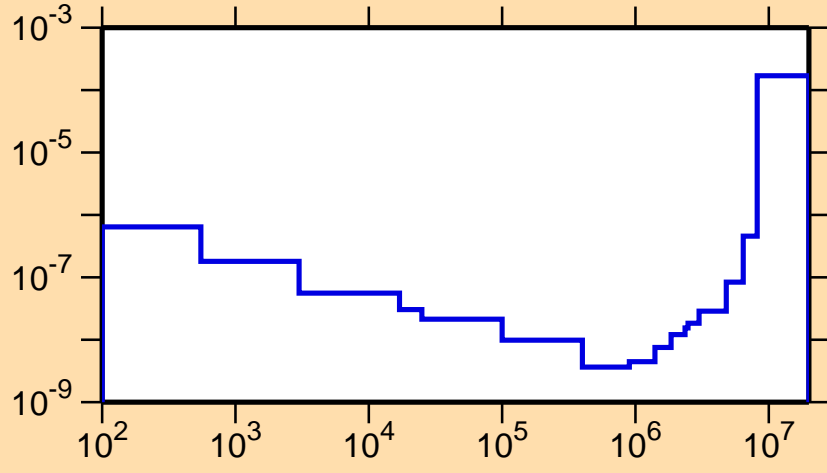
\sigma vs. E for ^{218}\text{Bi}(n,\alpha)
