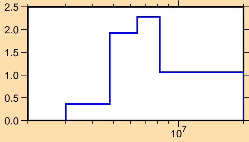
\sigma vs. E for ^{218}\text{Bi}(n,2n)
