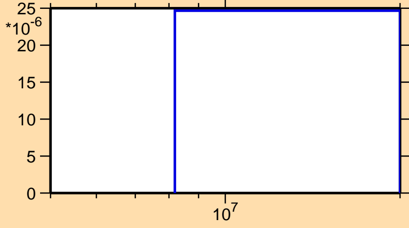
\sigma vs. E for ^{218}\text{Bi}(n,nt)
