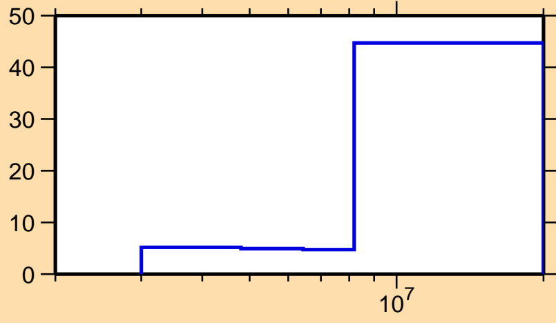
\Delta\sigma/\sigma vs. E for ^{218}\text{Bi}(n,2n)
