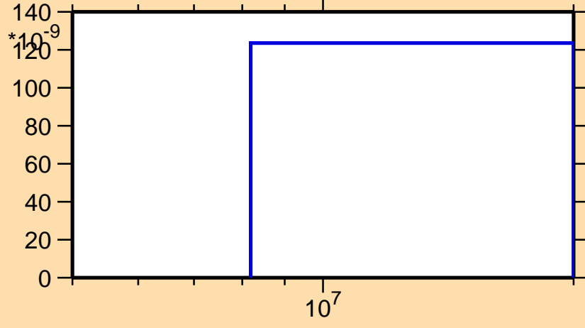
\sigma vs. E for ^{218}\text{Bi}(n,3n\alpha)
