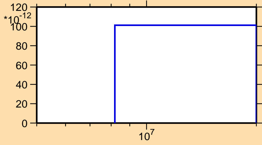
\sigma vs. E for ^{218}\text{Bi}(\text{mt } 11)
