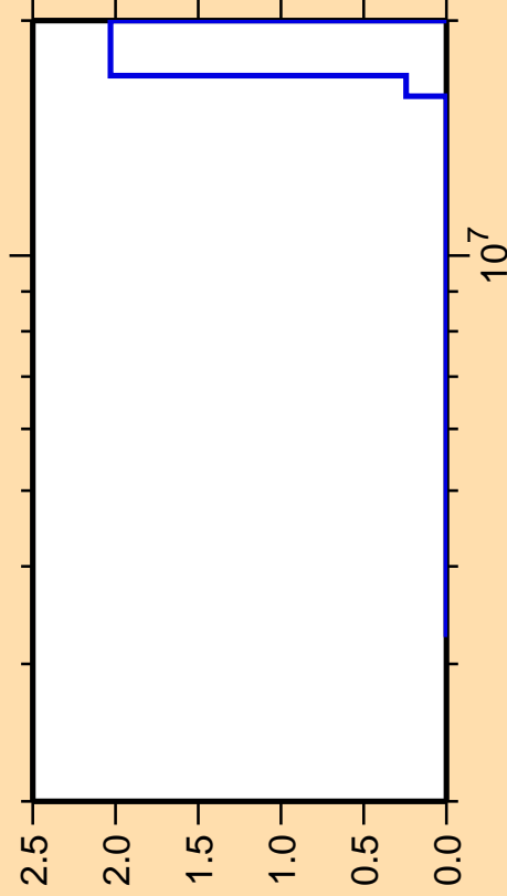
\Delta\sigma/\sigma vs. E for ^{220}\text{Bi}(n,f)
