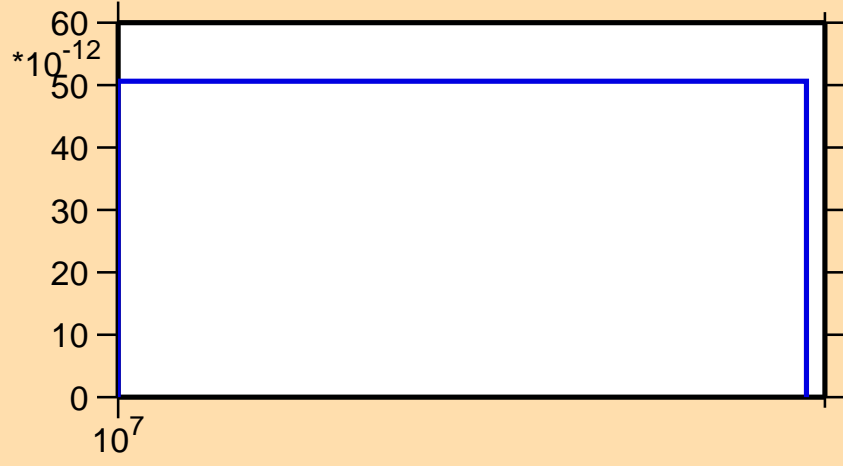
\sigma vs. E for ^{220}\text{Bi} (mt 11)
