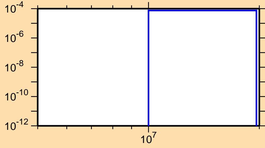
\sigma vs. E for ^{220}\text{Bi}(n,np)
