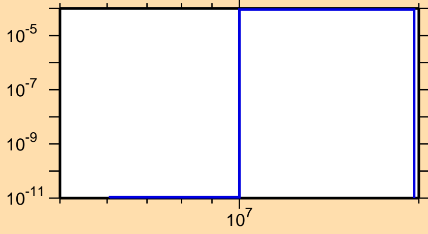
\sigma vs. E for ^{220}\text{Bi}(n,d)
