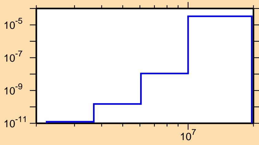
\sigma vs. E for ^{220}\text{Bi}(n,n\alpha)
