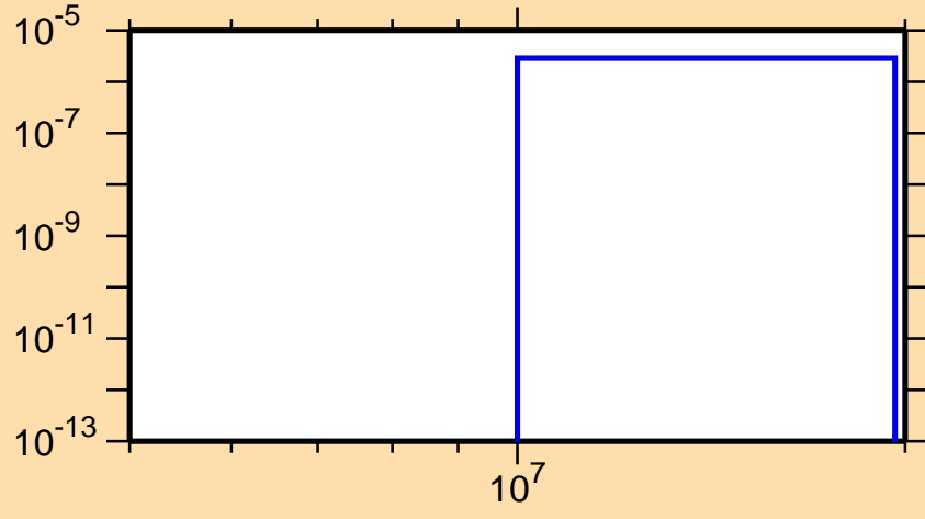
\sigma vs. E for ^{220}\text{Bi}(n,nd)
