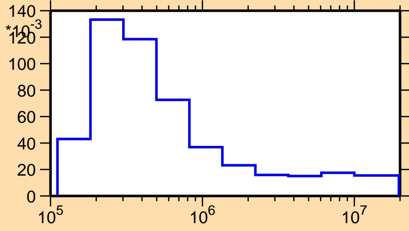
\sigma vs. E for ^{220}\text{Bi}(n,n_1)
