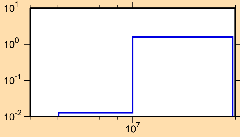
\sigma vs. E for ^{220}\text{Bi}(n,3n)
