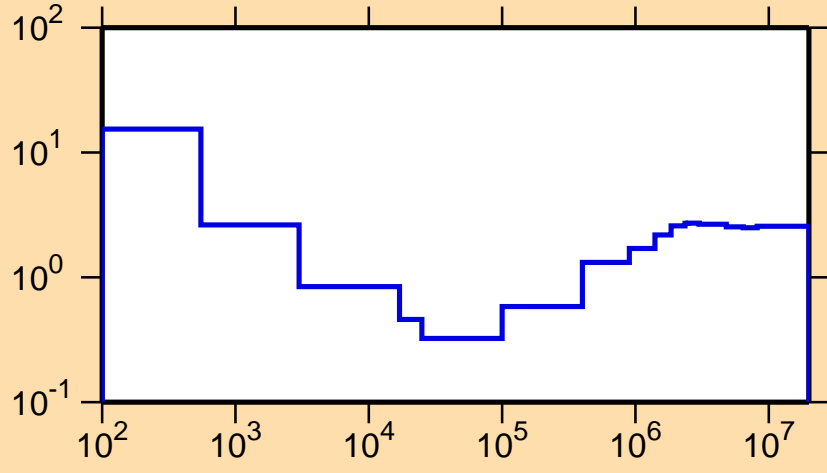
\sigma vs. E for ^{220}\text{Bi}(n,\text{nonel.})
