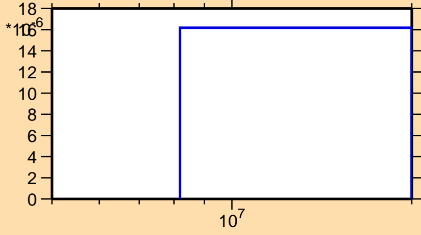
\sigma vs. E for ^{220}\text{Bi}(n,nt)
