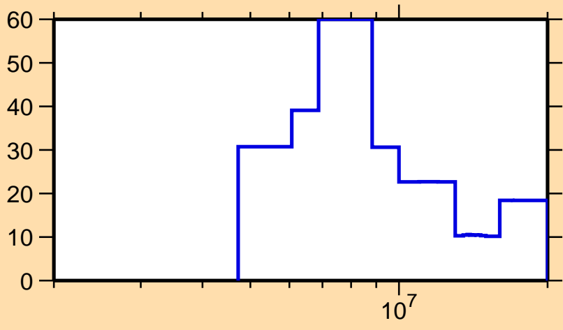
\Delta\sigma/\sigma vs. E for ^{221}\text{Bi}(n,\text{el.})
