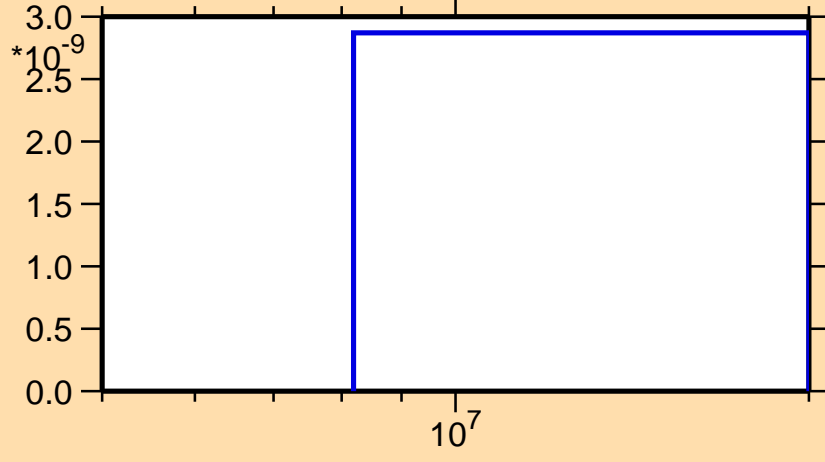
\sigma vs. E for ^{221}\text{Bi}(n,3n\alpha)
