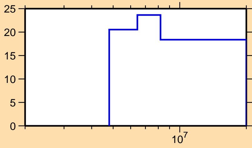
\Delta\sigma/\sigma vs. E for ^{221}\text{Bi}(n,\text{nonel.})
