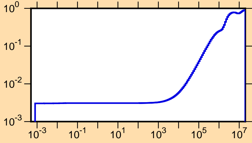
\mu vs. E for ^{222}\text{Bi}(\text{mt251})
