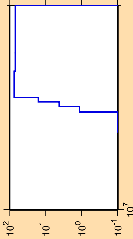
\Delta\sigma/\sigma vs. E for ^{222}\text{Bi}(n,2np)
