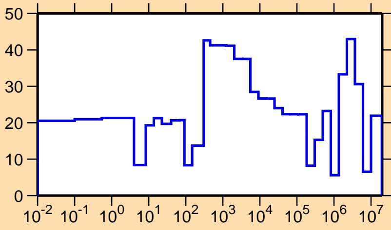
\Delta\sigma/\sigma vs. E for ^{222}\text{Bi}(n,el.)
