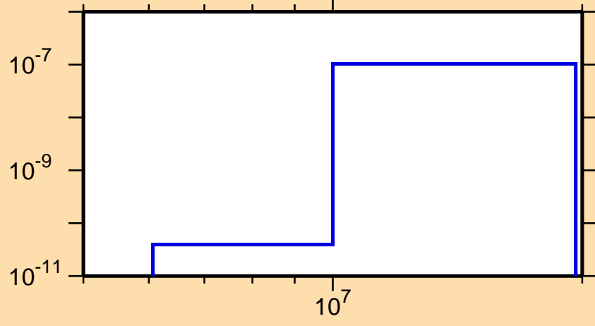
\sigma vs. E for ^{222}\text{Bi}(n,2n\alpha)
