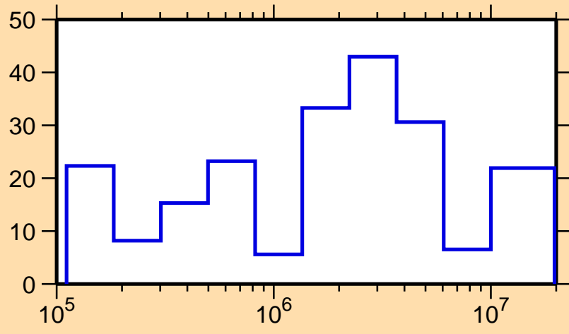
\Delta\sigma/\sigma vs. E for ^{222}\text{Bi}(n,\text{el.})
