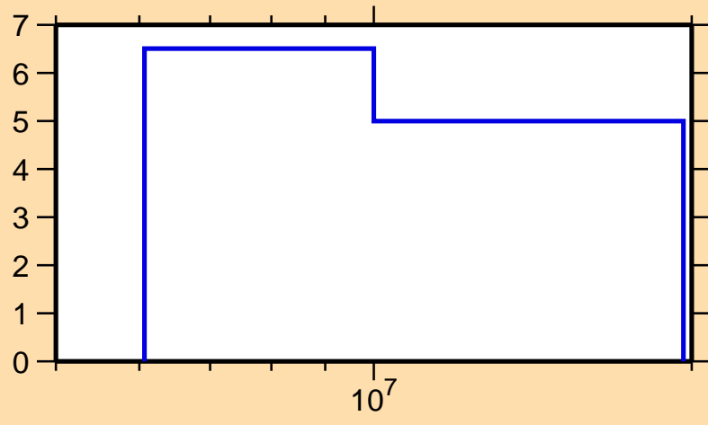
\Delta\sigma/\sigma vs. E for ^{222}\text{Bi}(n,\text{nonel.})
