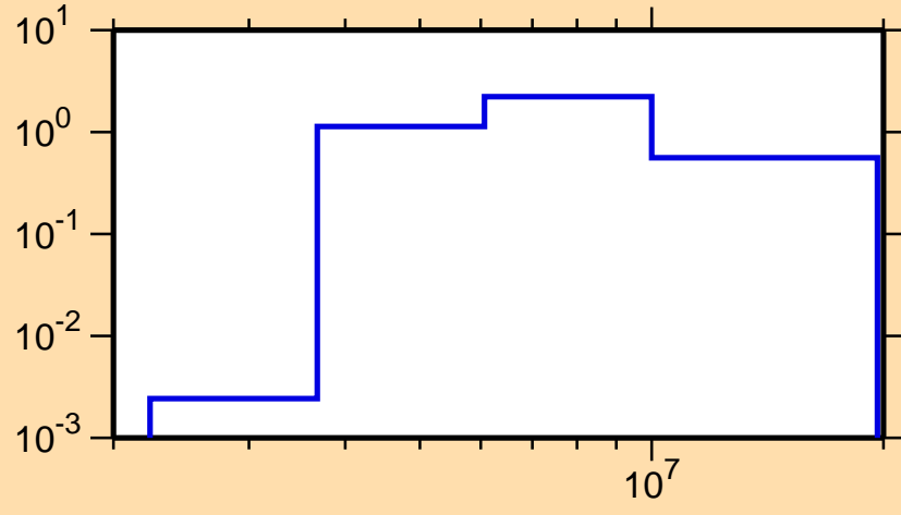
\sigma vs. E for ^{222}\text{Bi}(n,2n)
