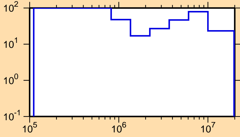
\Delta\sigma/\sigma vs. E for ^{222}\text{Bi}(n,n\text{cont.})
