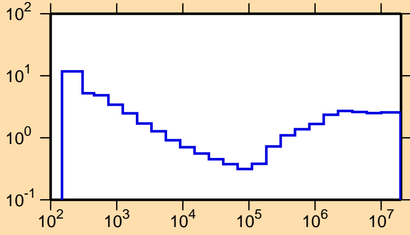
\sigma vs. E for ^{222}\text{Bi}(n,\text{nonel.})
