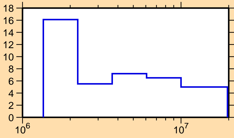
\Delta\sigma/\sigma vs. E for ^{222}\text{Bi}(n,\text{nonel.})
