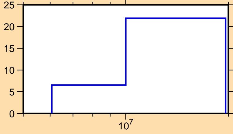
\Delta\sigma/\sigma vs. E for ^{222}\text{Bi}(n,el.)
