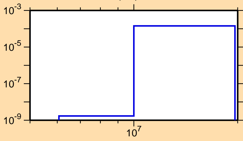
\sigma vs. E for ^{222}\text{Bi}(n,t)
