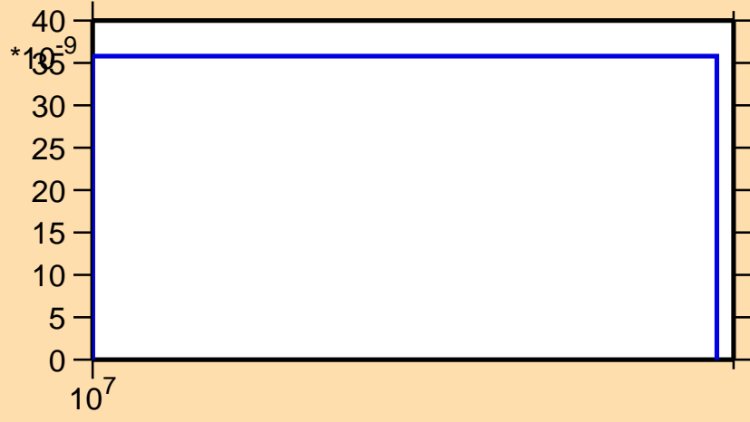
\sigma vs. E for ^{222}\text{Bi}(n,2np)
