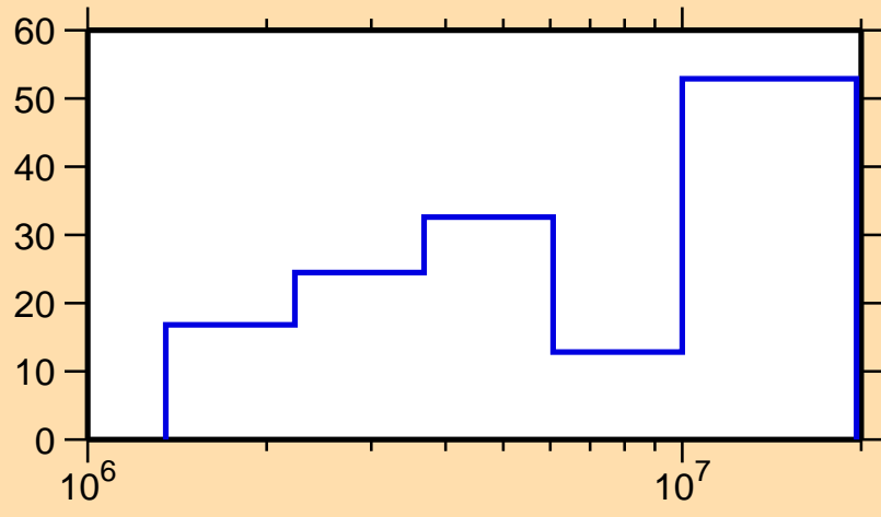
\Delta\sigma/\sigma vs. E for ^{222}\text{Bi}(n,\text{inel.})
