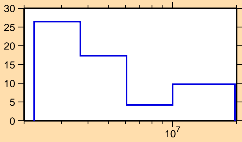
\Delta\sigma/\sigma vs. E for ^{222}\text{Bi}(n,\text{tot.})
