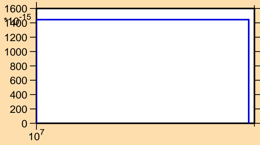
\sigma vs. E for ^{222}\text{Bi} (mt 11)
