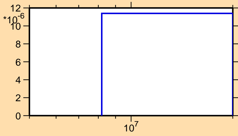
\sigma vs. E for ^{222}\text{Bi}(n,nt)
