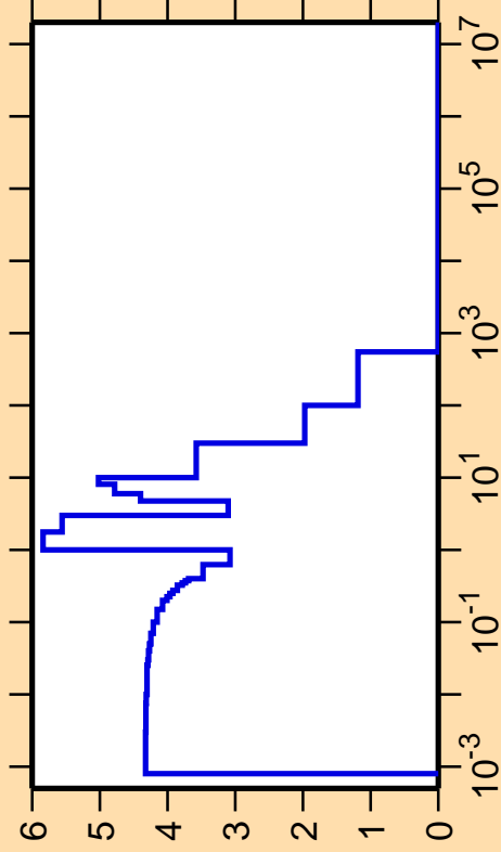
\Delta\sigma/\sigma vs. E for ^{222}\text{Bi}(n,f)
