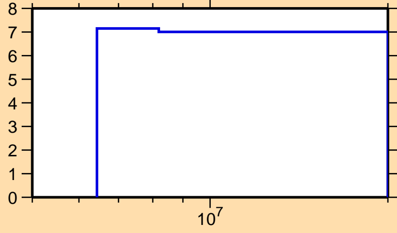
\Delta\sigma/\sigma vs. E for ^{222}\text{Bi}(n,\text{tot.})
