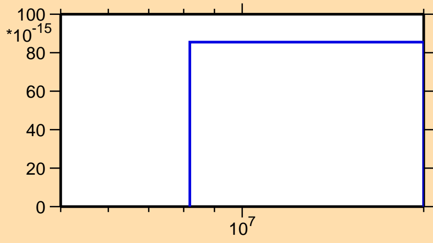
\sigma vs. E for ^{222}\text{Bi} (mt 42)
