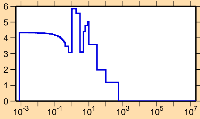
\Delta\sigma/\sigma vs. E for ^{222}\text{Bi}(n,f)
