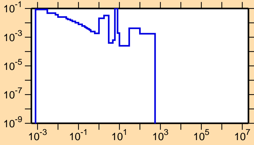
\sigma vs. E for ^{222}\text{Bi}(n,f)
