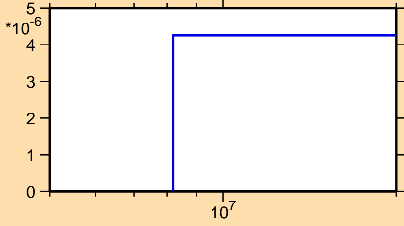
\sigma vs. E for ^{222}\text{Bi}(n,d)
