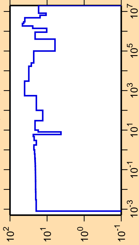
\Delta\sigma/\sigma vs. E for ^{222}\text{Bi}(n,\text{el.})
