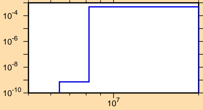
\sigma vs. E for ^{222}\text{Bi}(n,p)
