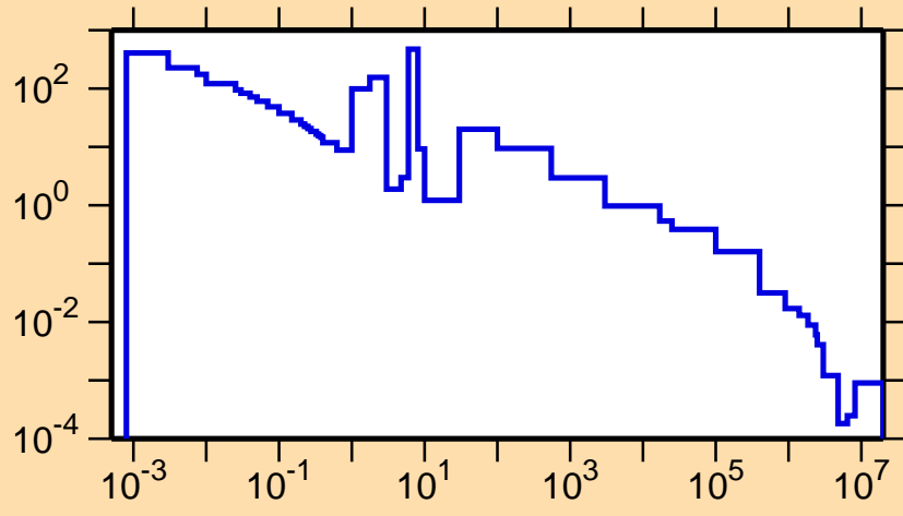
\sigma vs. E for ^{222}\text{Bi}(n,\gamma)
