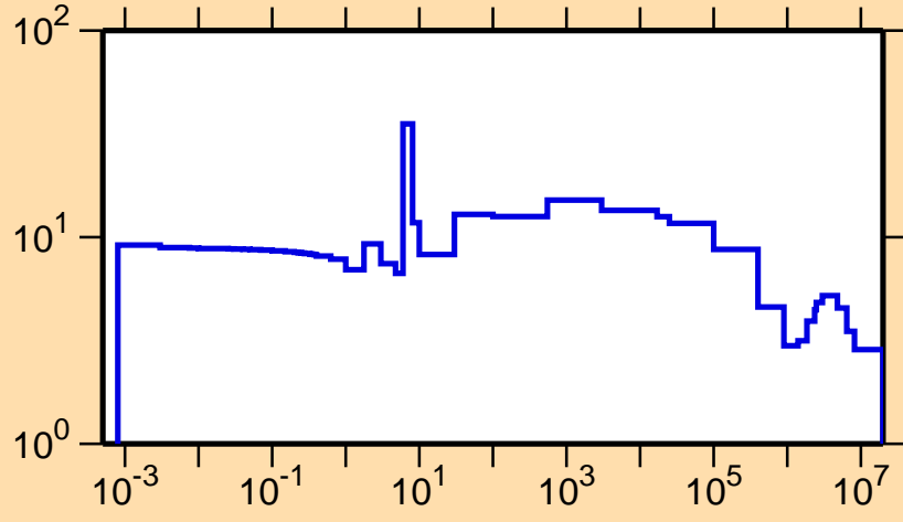
\sigma vs. E for ^{222}\text{Bi}(n,\text{el.})
