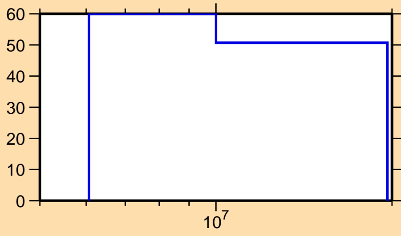
\Delta\sigma/\sigma vs. E for ^{223}\text{Bi}(n,\gamma)
