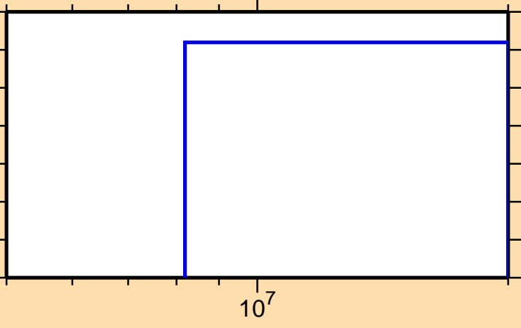
\sigma vs. E for ^{223}\text{Bi}(n,d)
