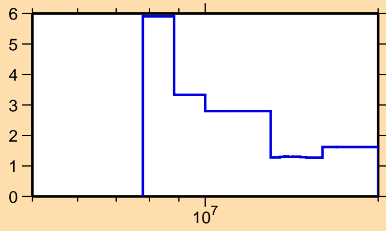
\Delta\sigma/\sigma vs. E for ^{235}\text{Bk}(n,\text{nonel.})
