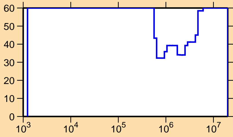
\Delta\sigma/\sigma vs. E for ^{235}\text{Bk}(n,p)
