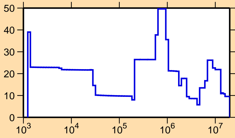
\Delta\sigma/\sigma vs. E for ^{235}\text{Bk}(n,el.)
