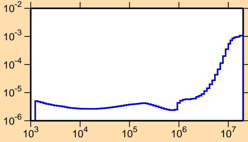
\sigma vs. E for ^{235}\text{Bk}(n,\alpha)
