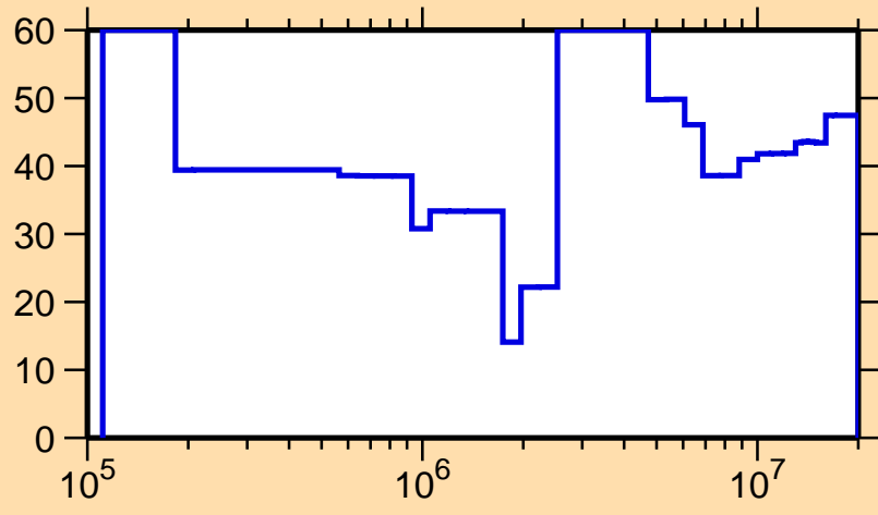
\Delta\sigma/\sigma vs. E for ^{235}\text{Bk}(n,n_1)
