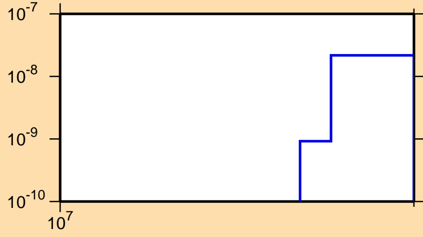
\sigma vs. E for ^{235}\text{Bk}(n,3n\alpha)
