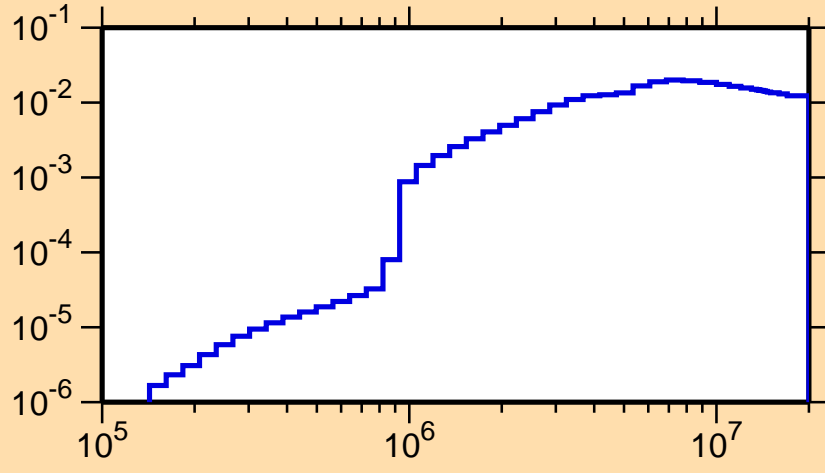
\sigma vs. E for ^{235}\text{Bk}(n,n\alpha)
