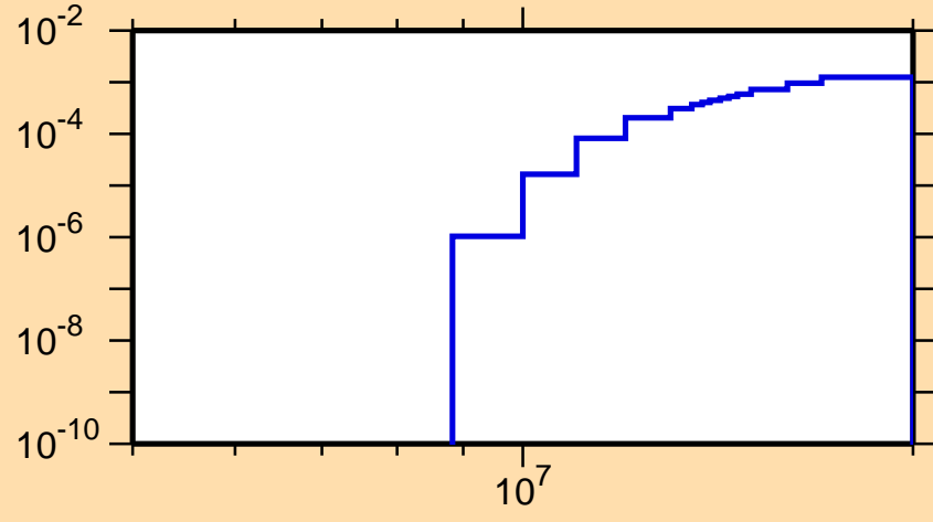
\sigma vs. E for ^{235}\text{Bk}(n,2n)
