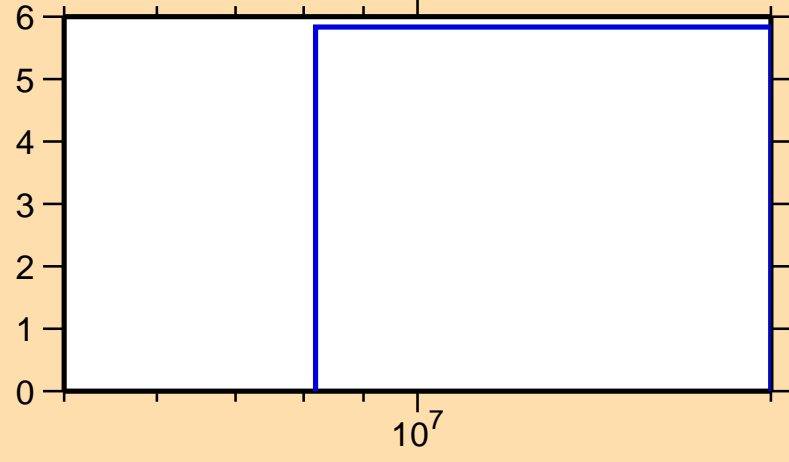
\Delta\sigma/\sigma vs. E for ^{235}\text{Bk}(n,\text{tot.})
