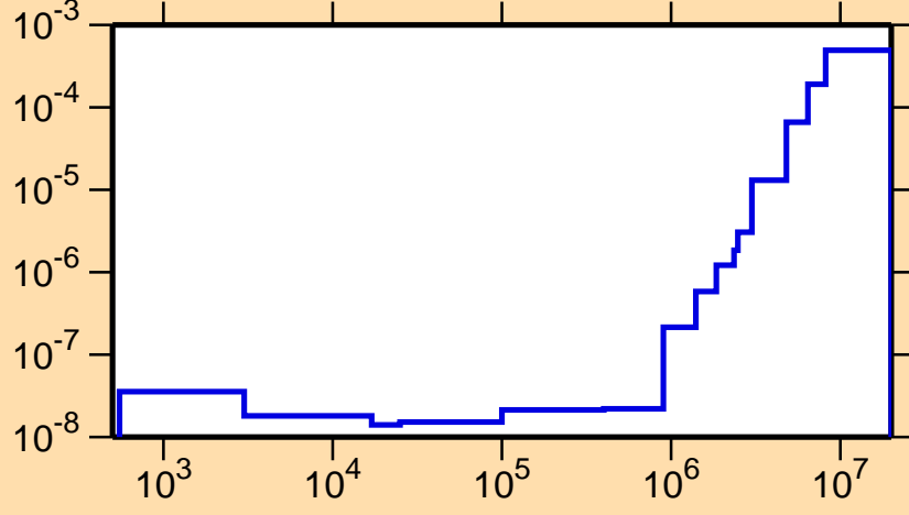
\sigma vs. E for ^{235}\text{Bk}(n,p)
