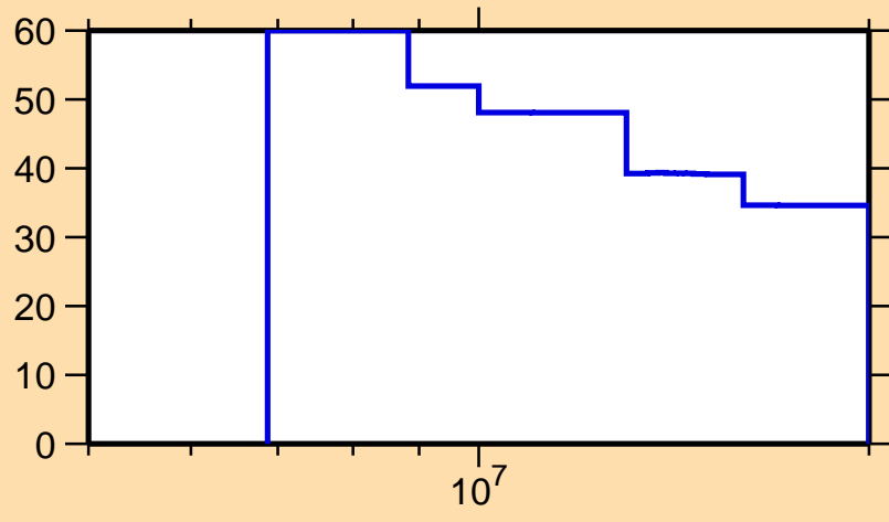
\Delta\sigma/\sigma vs. E for ^{236}\text{Bk}(n,2n)
