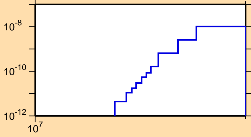
\sigma vs. E for ^{236}\text{Bk}(n,nd)
