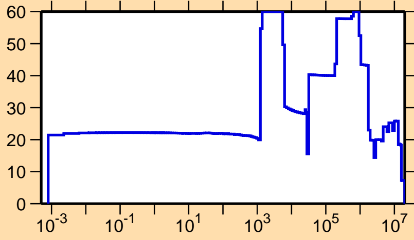
\Delta\sigma/\sigma vs. E for ^{236}\text{Bk}(n,el.)
