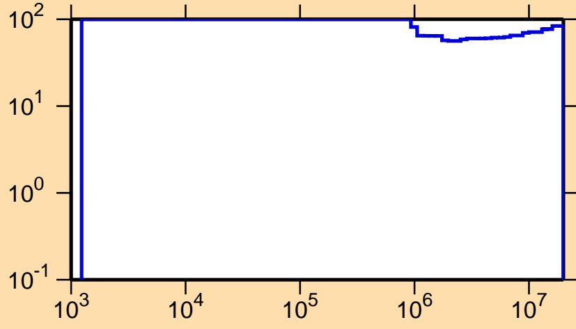
\Delta\sigma/\sigma vs. E for ^{236}\text{Bk}(n,p)
