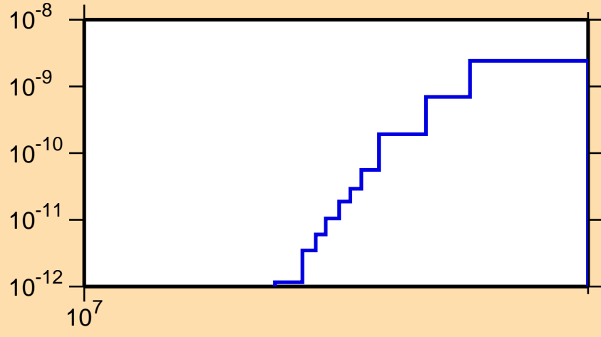
\sigma vs. E for ^{236}\text{Bk}(n,2np)
