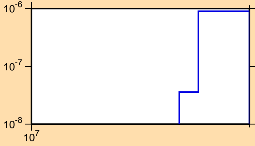
\sigma vs. E for ^{236}\text{Bk}(n,3n\alpha)
