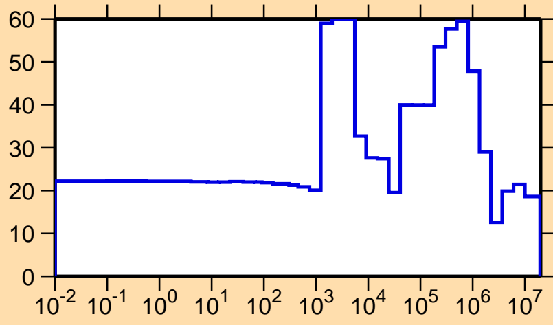
\Delta\sigma/\sigma vs. E for ^{236}\text{Bk}(n,el.)
