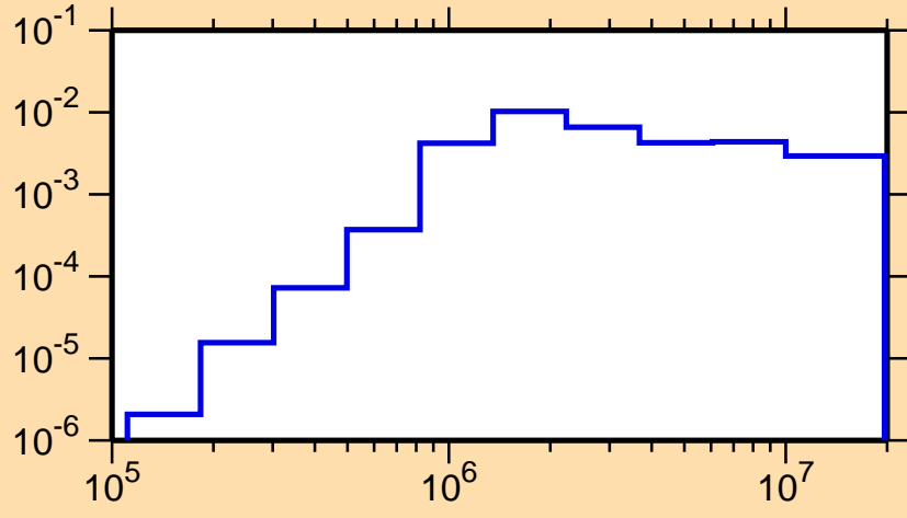
\sigma vs. E for ^{236}\text{Bk}(n,\text{inel.})
