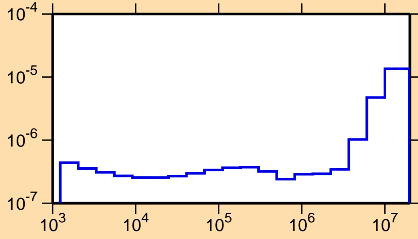
\sigma vs. E for ^{236}\text{Bk}(n,\alpha)
